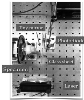
Figure 4.—Experimental apparatus: (a) schematic diagram and (b) photographic view.
