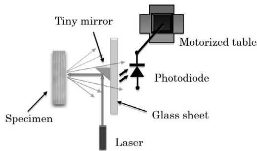
Figure 4.—Experimental apparatus: (a) schematic diagram and (b) photographic view.
