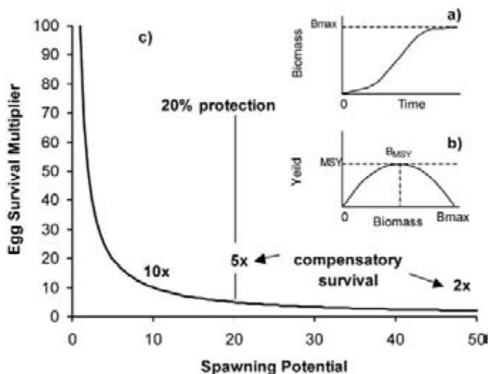
Figure 8. Recruitment and minimum levels of reserve protection. The logistic population growth curve a ) in which fastest growth is achieved when the population is at about half of its maximum level ( B_{max} ) is the basis for the principle of maximum sustainable yield (MSY). At higher levels of biomass population growth slows due to density dependent effects on the survivorship or growth of recruits. The New Zealand Fisheries Act 1996 requires fisheries to be managed so that they are at the B_{MSY} level b ), forming the basis of setting TAC in all quota management species. In a population harvested down to B_{MSY} approximately 50% of the original spawning potential (egg production) of the population would remain, but reduced egg production is expected to be compensated for by a two-fold increase in egg survival due to release from density dependent effects c ). Reducing the population to smaller and smaller fractions of its spawning potential, requires a corresponding increase in egg survival in order to maintain the original spawning potential and sustainable harvest. At levels at or below 20% of spawning potential the increases in egg survival required begin to exceed those that might be realistically expected (i.e. 5 – 10 fold increases). It has been argued by Bohnsack (2003) that protecting at least 20% of a species' habitat in reserves will provide insurance that at least that much of the spawning potential remains.
