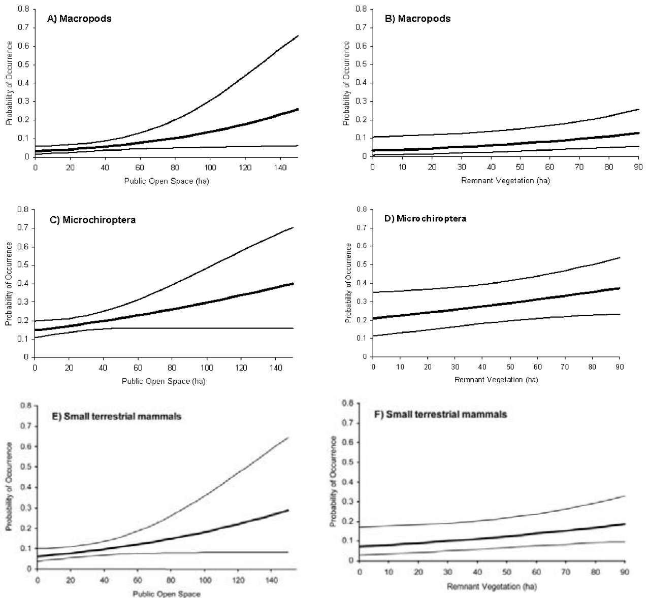
Figure 4. Logistic regression model of the occurrence of species of macropod ( \text{logit}(p) = -3.458 + 0.004 \text{ VEG} + 0.016 \text{ OS} ); microchiropteran species ( \text{logit}(p) = -1.824 + 0.020 \text{ VEG} + 0.009 \text{ OS} ); and small ground-dwelling mammals ( \text{logit}(p) = -2.727 + 0.007 \text{ VEG} + 0.012 \text{ OS} ) as a function of the amount of remnant vegetation (VEG) and public open space (OS) within a 700 m radius of each grid cell. a), c), e) Effect of public open space, with remnant vegetation set at its mean (3.42 ha); b), d), f) Effect of remnant vegetation, with public open space set at its mean (24.5 ha).
