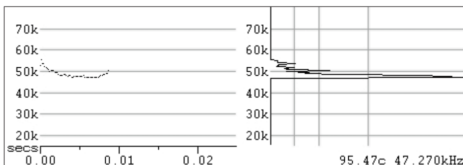
Figure 15: Frequency versus time graph (left) and duty cycle (right) of a typical call pulse from Mormopterus cf. beccarii in the 44–50 kHz harmonic recorded in the flight enclosure at Akwam 3/4/03. Scale: real time, 5 ms per tick (F8 and TBC uncompressed in Analook).
