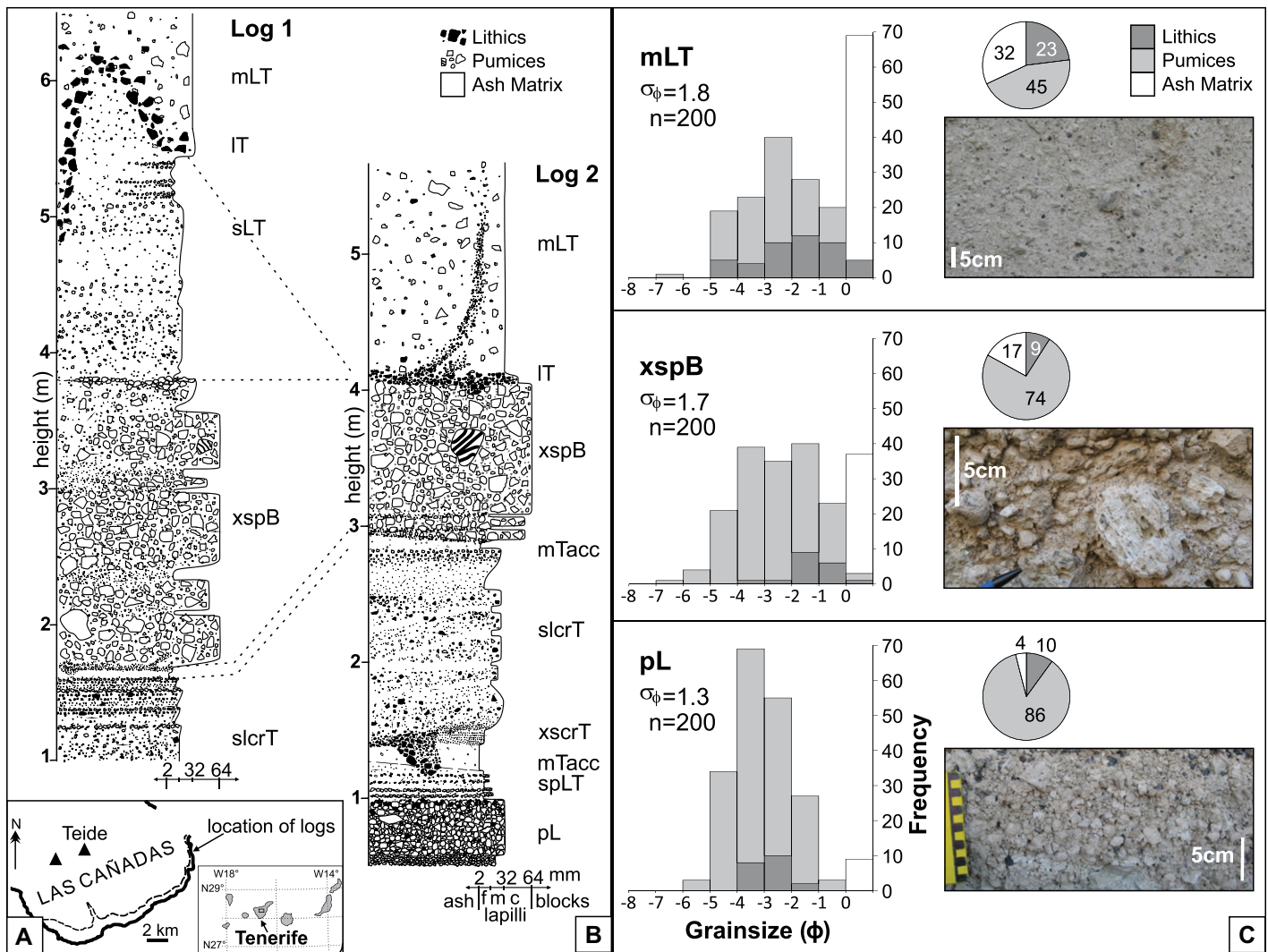
Figure 1. The xspB facies, Tenerife, Canary Islands. (A) Location, and (B) stratigraphic logs 20 m apart at 28.280273°N, 16.549526°W. Facies abbreviation key is shown in Figure 3. (C) Grain size distribution histograms and pie charts illustrating comparative grain size, sorting, and componentry (see the Supplemental Material 1 ).
