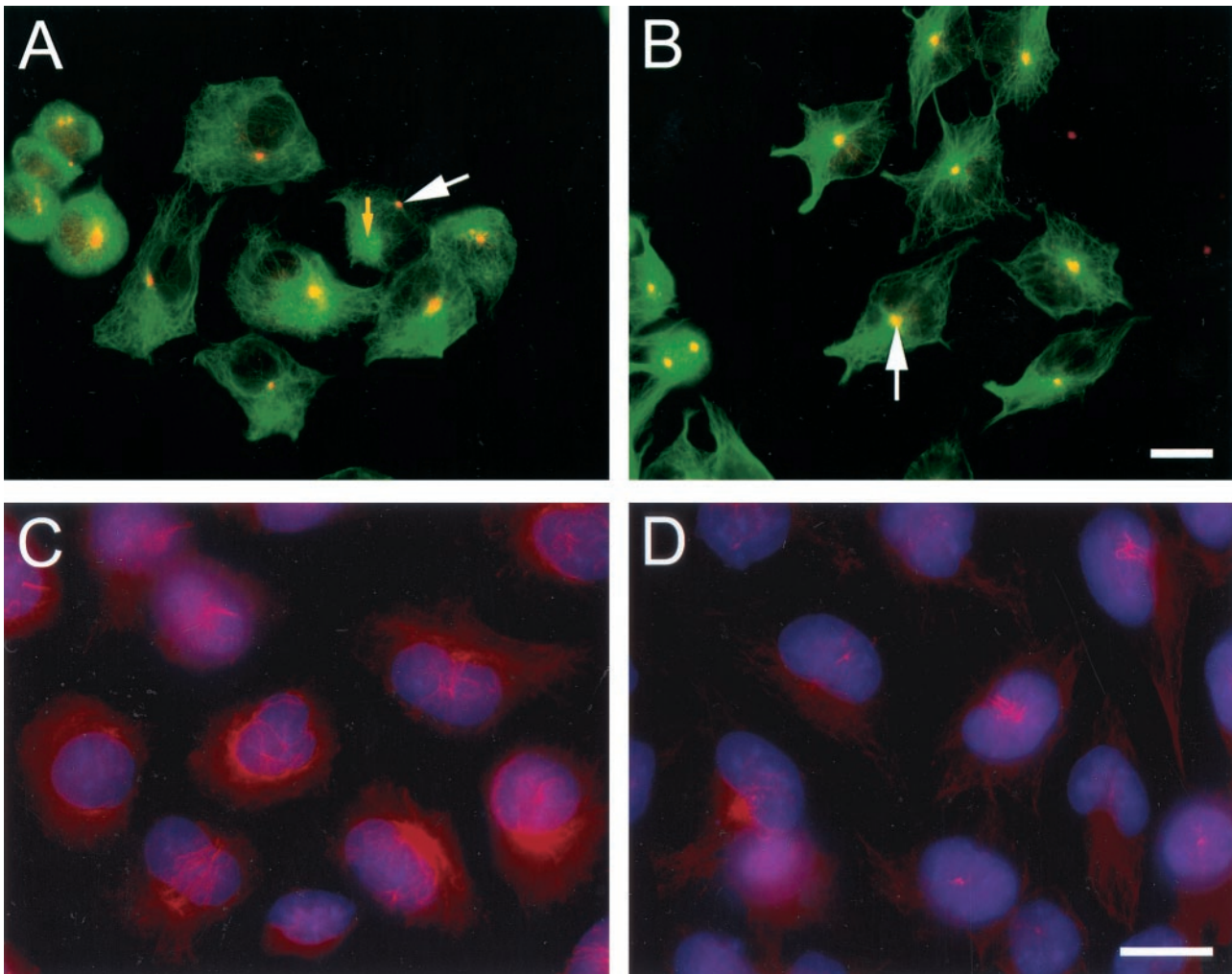
Fig. 3. Effects of CP248 on interphase 9L cells. The 9L cells were treated with 0.075 \mu\text{M} CP248 (A, C) or 0.1% DMSO (B, D) for 6 h, fixed with methanol; and DNA, MTs, and centrosomes were visualized by indirect immunofluorescence, as described in Fig. 2 and “Materials and Methods.” In B, DMSO-treated 9L cells show a tight correlation of centrosomes (stained red) with the MT array (white arrow). In A, CP248-treated 9L cells show a dissociation of the centrosome (white arrow) from the MT array (yellow arrow). In C, CP248-treated 9L cells were stained for stable Glu MTs (red) and DNA (blue). In D, DMSO-treated 9L cells were stained for stable Glu MT (red) and for DNA (blue). White bars, 20 \mu\text{m} .
