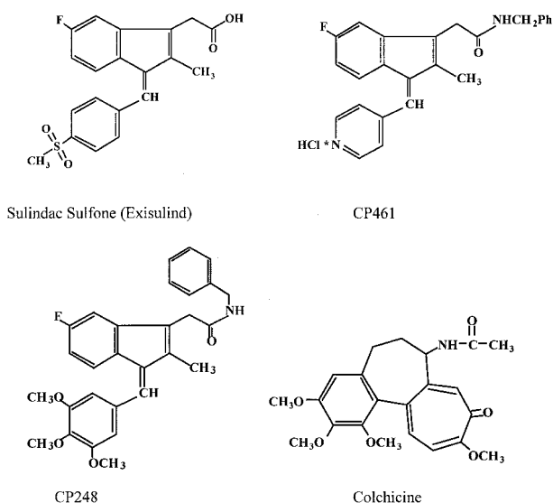
Fig. 1. Chemical structures of exisulind, CP461, CP248, and colchicine.
