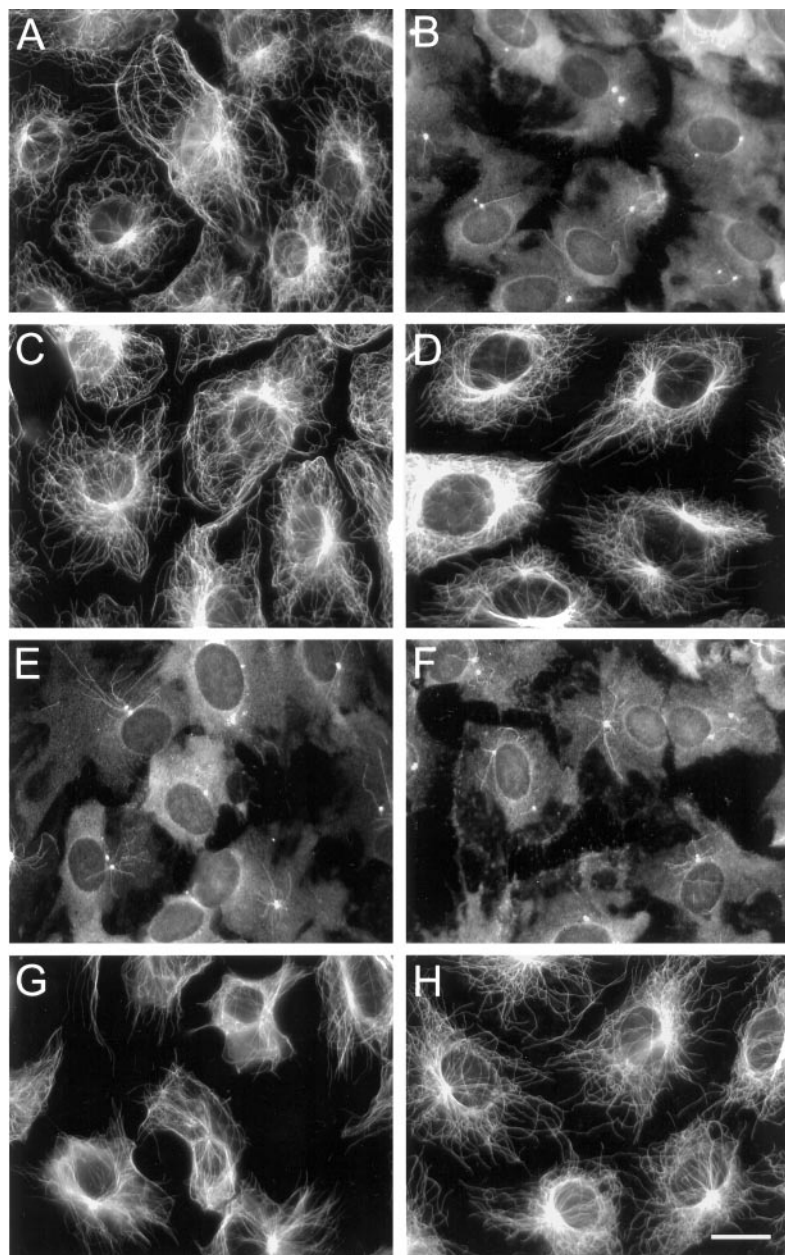
Fig. 5. Effects of CP248 on MTs in NIH 3T3 fibroblasts. The cells were grown in medium in the absence of serum for 48 h. They were then incubated in medium minus serum containing: 0.1% DMSO (A); 0.1 \mu\text{M} CP248 (B); 200 \mu\text{M} exisulind (C); 1.5 \mu\text{M} CP461 (D); 0.1 \mu\text{M} CP248 plus 10 \mu\text{M} KT5823 (E); 0.1 \mu\text{M} CP248 plus 10 \mu\text{M} Rpt-8-pCPT0cGMP (F); 170 nM YC-1 (G); or 4 mM dibutyryl cGMP (H). After 2 h of incubation with these agents, the cells were fixed with methanol and the MTs visualized by immunofluorescence, as described in "Materials and Methods." White bars, 20 \mu\text{m} .
