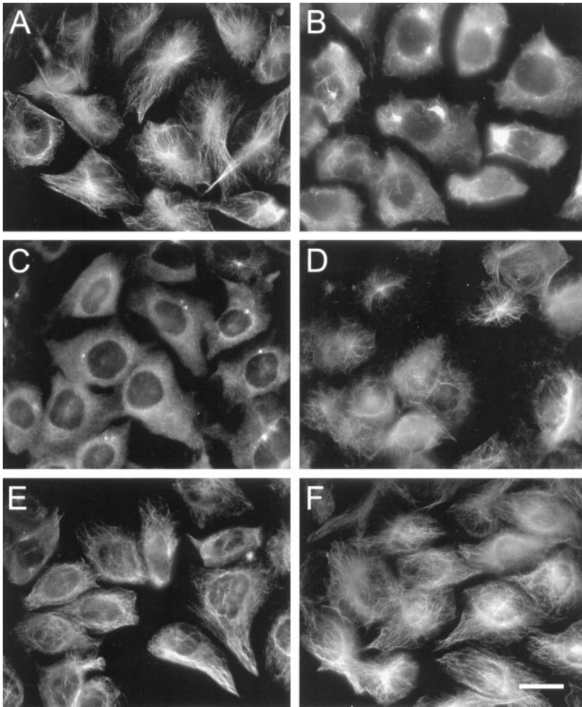
Fig. 4. Effects of CP248 on MTs in interphase 9L cells. 9L cells were treated with 0.1% DMSO (A), 0.2 \mu\text{M} CP248 (B), or 0.4 \mu\text{M} CP248 (C) for 2 h. The cells were fixed with methanol, and MTs were visualized by immunofluorescence, as described in “Materials and Methods.” The 9L cells were treated with 0.4 \mu\text{M} CP248 for 2 h, washed three times with fresh medium, and then incubated for an additional 15 (D), 30 (E), or 60 (F) min, before fixation and immunostaining. White bars, 20 \mu\text{m} .
