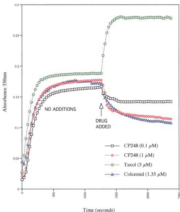
Fig. 6. Effects of CP248 on in vitro MT polymerization, measured by turbidity. A solution of MTs at 4°C was placed into a thermostable chamber of a spectrophotometer and incubated at 37°C. Absorbance at 350 nm was then determined during the indicated time course. After MT polymerization reached a steady state (20 min), 5 \mu\text{M} Taxol, 0.1 \mu\text{M} CP248, 1 \mu\text{M} CP248, or 1.35 \mu\text{M} Colcemid were added. Because Colcemid and CP248 gave some absorbance at 350 nm, this value was subtracted from the total absorbance. For additional details, see "Materials and Methods."
