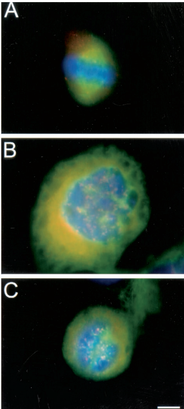
Fig. 2. Effects of CP248 on mitotic 9L cells. A , a mitotic 9L cell after treatment with 0.1% DMSO (solvent control). B , a 9L cell treated with 50 ng/ml Colcemid (positive control). C , a mitotic 9L cell after treatment with 0.075 \mu\text{M} CP248. Cells were treated for 12 h and fixed with methanol. Chromosomal DNA was stained blue with DAPI. MTs were stained green and MAD2 proteins were stained red with the respective antibodies and were visualized by indirect immunofluorescence, as described in "Materials and Methods." Abnormal spindle apparatus is notable in the CP248-treated cells. White bar, 10 \mu\text{m} .
