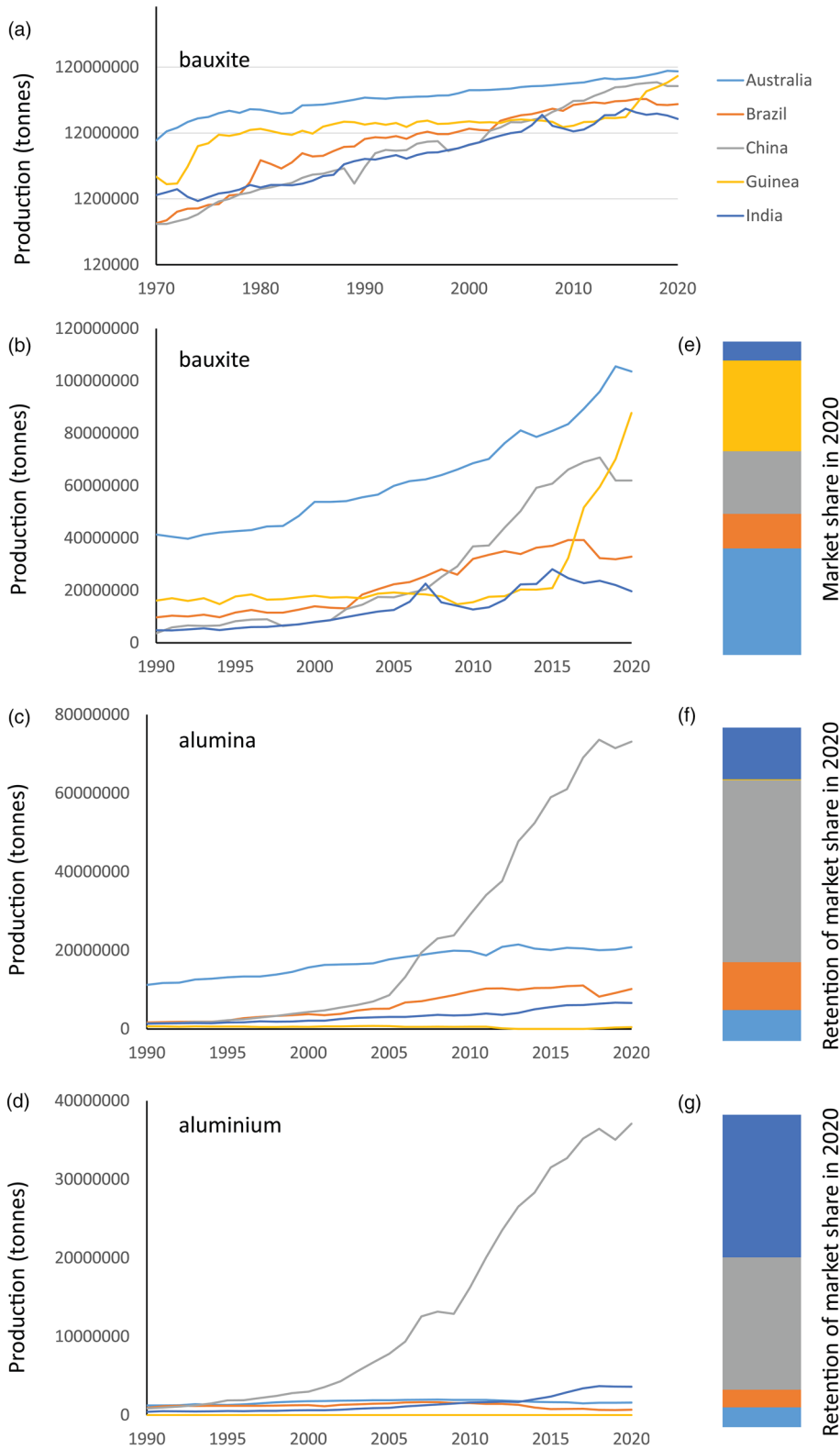
Fig. 5. Production in Australia, Brazil, China, Guinea and India of (a, b) bauxite, (c) alumina and (d) aluminium. The long-term production data shows a relatively consistent rate of increase prior to 1995, at which point production and consumption accelerate markedly. The market share between the top 5 producers is normalized to 100% in (e), for the purposes of depicting retention of mineral wealth within country. The retention of mineral wealth within country is indicated for the top 5 producers as a scaled bar for alumina relative to bauxite (f) and primary aluminium relative to alumina (g), derived from ratios of commodity production data. All figures derived using data from the World Mineral Production mineral statistics database (British Geological Survey 2023).
