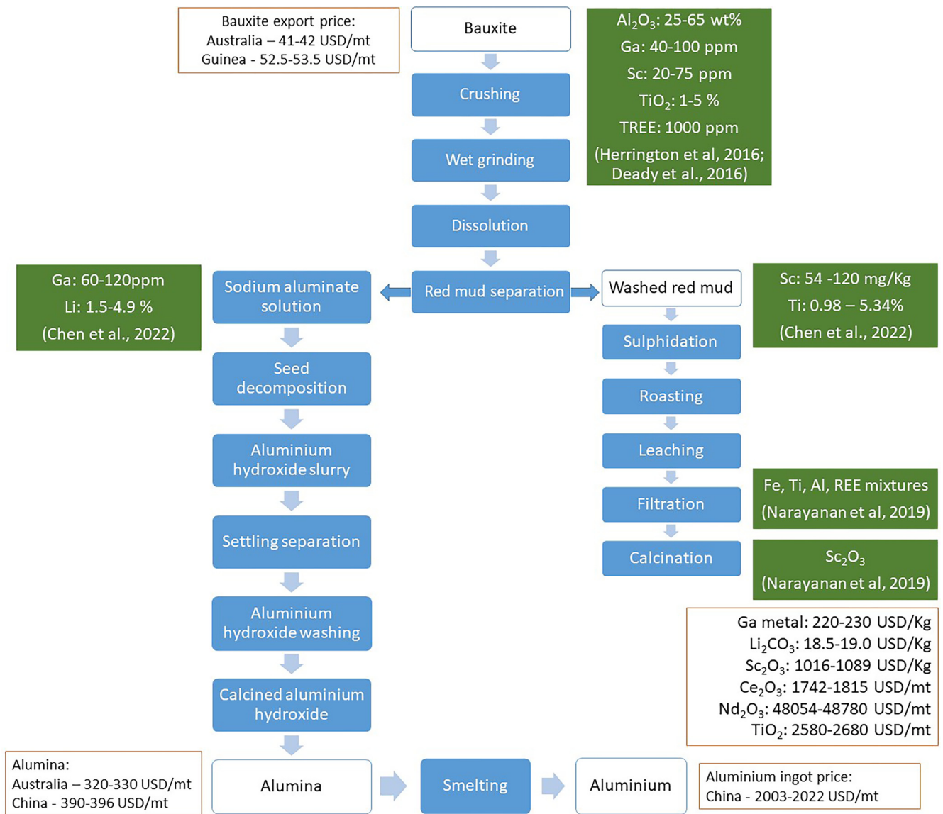
Fig. 4. Schematic overview of the recovery process of intermediate products and by-products between bauxite and aluminium, showing that the high value products are produced at sites of alumina production and aluminium smelting rather than at the location of bauxite production. The simplified Bayer and additional processes (excluding hydrolysis, chlorination and pyrometallurgy) are based on the various extraction schemes and flowsheets of: Borra et al. (2016); Onghena et al. (2017); Narayanan et al. (2019); Chen et al. (2022). The concentrations of major and minor components in bauxite and red mud are from: Deady et al. (2016); Herrington et al. (2016). The commodity prices are quoted as US$/metric tonne (USD/mt) or as US$.kilogram (USD/kg) and sourced from the Institute of rare earth elements and strategic metals: https://en.institut-seltene-erden.de/aktuelle-preise-von-basismetallen/ (commodity price correct, 5 December 2022). Products such as aluminium fluoride and aluminium alloys have commodity prices of 1370–1441 and 1460–2085 USD/mt, respectively.
