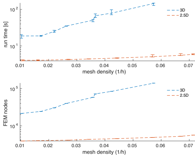
Figure 9. The 2.5-D Jacobian calculations scale with FEM node count: the 2.5-D movement Jacobian speed advantage over a rank-one 3-D calculation (Gómez-Laberge & Adler 2008) grows as mesh density (FEM elements per metre) 1/h , where h is the maximum element height for the entire mesh. Error bars show max/min run times over 20 runs, the run time is closely related to the number of nodes in the FEM mesh where 2-D meshes have far fewer nodes for the same mesh density.
