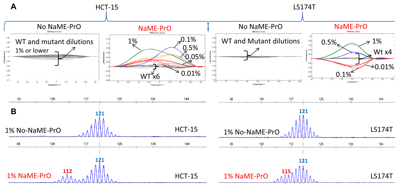
Figure 2. NaME-PrO application on BAT25 microsatellite in serial dilutions of DNA from MSI-H cell lines. (A). Comparison between NaME-PrO-treated and untreated DNA for BAT25 microsatellites on DNA from colon cancer cell lines HCT15 (left) and LS174T (right) serially diluted into WT DNA, detected via high resolution melting. (B) Capillary electrophoresis analysis for 1% DNA abundance FOR HCT-15 DNA (left) and LS174T DNA (right) (red = variant, blue = WT).
