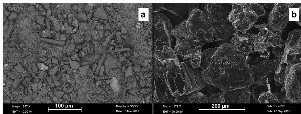
FIG. 4. (a) A BSEM image (from VPSEM) of mudstone starting material showing fine silt particles accumulated within the channel formed by the "ridge and furrow" lineaments on the fracture surface. (b) A SEM image of sandstone starting material showing euhedral authigenic K-feldspar and quartz overgrowth cements with some illite–smectite clay coating on detrital quartz grains (courtesy of A. E. Milodowski, BGS).
