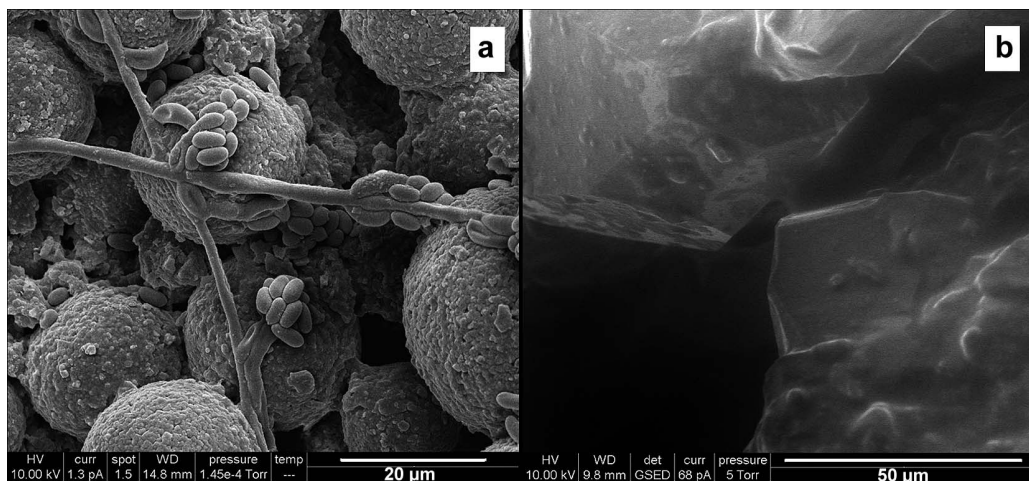
FIG. 5. (a) A CryoSEM SEI image showing detail of the clusters of rod-like cells associated with the biofilm resting on fresh framboidal pyrite in the reacted mudstone. High-vacuum cryoSEM, gold coated sample, FEI ESEM instrument (courtesy of A. E. Milodowski, BGS). (b) An ESEM SEI image of reacted sandstone showing the largely planar pore walls to a macropore covered by P. aeruginosa derived biofilm which is darker in its colouration and locally bridges smaller gaps (above and right of centre) (courtesy of J. Rushton, BGS).
