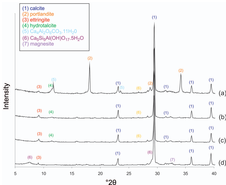
FIG. 1. X-ray diffraction patterns for (a) untreated NRVB; (b) NRVB leached for 541 days; (c) NRVB leached for 1272 days; and (d) NRVB subjected to leaching followed by hydrothermal treatment, with principal peaks indicated.
