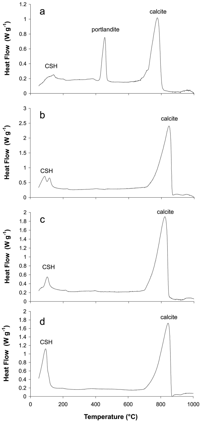
FIG. 2. Differential scanning calorimetry traces for (a) untreated NRVB; (b) NRVB leached for 541 days; (c) NRVB leached for 1272 days; and (d) NRVB subjected to leaching followed by hydrothermal treatment.
