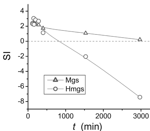
FIG. 2. Saturation index as a function of time calculated using PHREEQC from experimental data obtained in the 180°C series.
