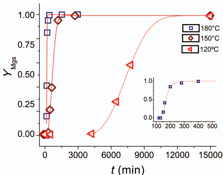
FIG. 4. Fitting of the experimental points to the Avrami equation for the three working temperatures.
