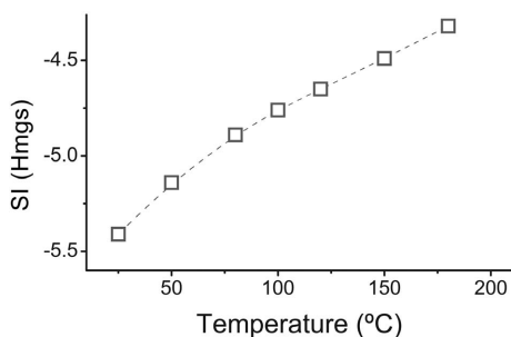
FIG. 3. Saturation index of hydromagnesite in an aqueous solution saturated with respect to magnesite at different temperatures.
