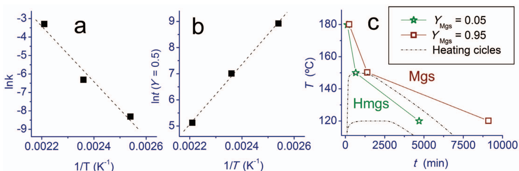
FIG. 5. (a) Linear fitting of \ln k vs. the reciprocal of temperature expressed in Kelvin. (b) Linear fitting of \ln t_{Y=0.5} vs. the reciprocal of temperature in Kelvin. (c) TTT graph of the transformation process of hydromagnesite to magnesite. The dashed lines indicate two hypothetical heating cycles.
