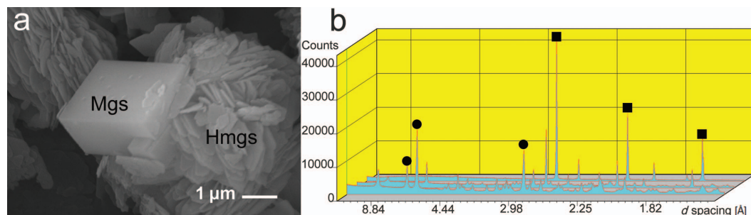
FIG. 1. (a) SEM image of magnesite and hydromagnesite at: T = 180^\circ\text{C} , t = 160 min. (b) Schematic representation of the powder-XRD identification of the transformation process. ■: most intense reflections of magnesite – 2.74 Å (104), 2.10 Å (113), 1.69 Å (108). ●: most intense reflections of hydromagnesite – 9.21 Å (100), 5.80 Å (011), 2.90 Å (12̄2). The XRD patterns correspond to 120, 200 and 2970 min of reaction time, respectively, from front to rear.
