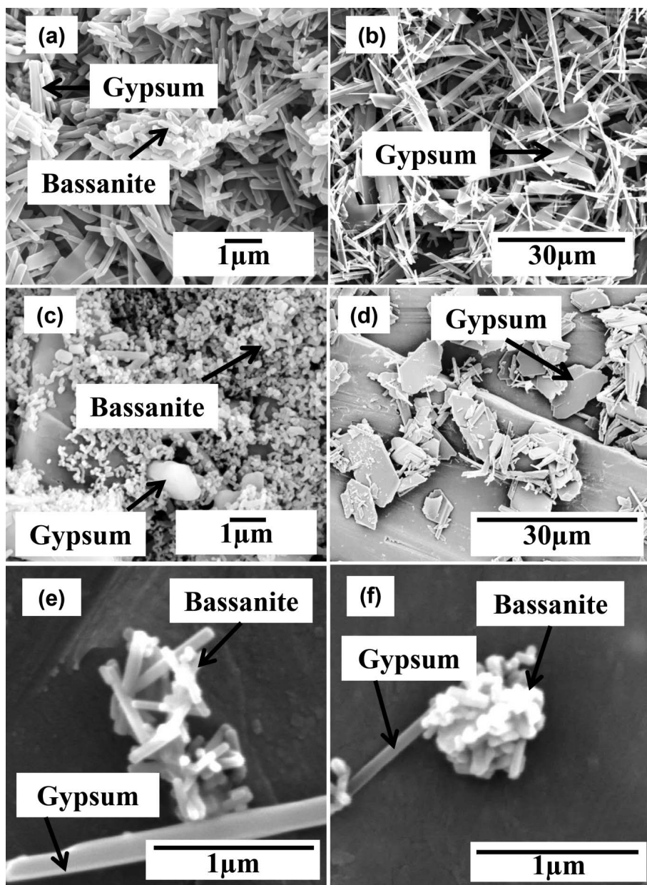
FIG. 4. SEM image of precipitated materials from experiments in: (a) the pure CaSO 4 system 30 s after turbidity onset showing bassanite nanorods and gypsum needles; (b) the pure CaSO 4 system 63 min after turbidity onset (70 minutes total time) showing only variably sized gypsum needles; (c) tiny bassanite nanoparticles formed in the presence of 20 ppm citric acid 3 min after turbidity onset together with some larger gypsum crystals; (d) plate-like gypsum crystals formed in the presence of 20 ppm citric acid after 200 min of total reaction; (e) bassanite nanorods and a single larger gypsum needle collected a few minutes after the onset of turbidity in the 20 ppm maleic acid experiment; (f) bassanite nanorods and a single larger gypsum needle collected a few minutes after the onset of turbidity in the 20 ppm tartaric acid experiment.
