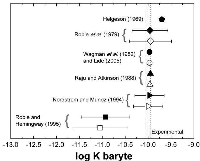
FIG. 1. Calculated log K for baryte solubility at the 95% confidence limit, determined from the Gibbs free energy of reaction, derived from two approaches: (a) from enthalpy and entropy (filled symbols); and (b) from Gibbs free energy of formation (open symbols). Values from Helgeson (1969), Wagman et al. (1982), Lide (2005) and Raju and Atkinson (1988) were reported without uncertainty. The double dotted vertical bar represents the range of experimental values for the logarithm of the thermodynamic solubility product for baryte (log K: -10.05 to -9.96 ).
