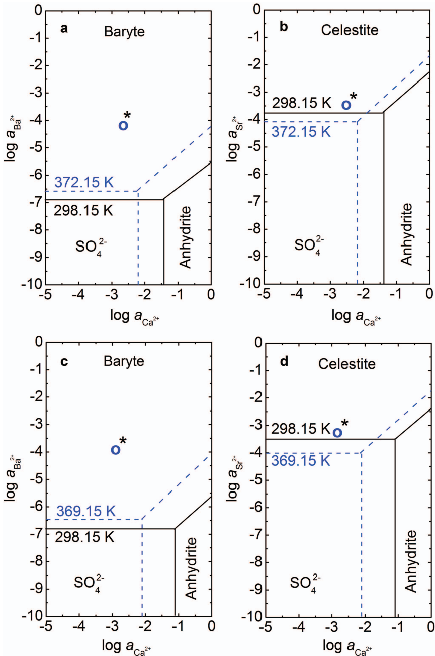
FIG. 2. Activity-activity diagram for the Beryll and Forties Field: (a) The \text{Ba}^{2+} - \text{Ca}^{2+} - \text{SO}_4^{2-} and (b) the \text{Sr}^{2+} - \text{Ca}^{2+} - \text{SO}_4^{2-} systems at atmospheric pressure, 298.15 K (with \log a_{\text{SO}_4^{2-}} = -3.011 ) and 372.15 K (with \log a_{\text{SO}_4^{2-}} = -2.975 ) for a solution of equal portions of seawater and Beryll Field formation water. The bold star represents the mixed water composition at 298.15 K (c) and the blue open circle at 372.15 K. (c) and (d) Similar diagrams for the same systems with solubility predicted for temperatures of 298.15 K (with \log a_{\text{SO}_4^{2-}} = -3.157 ; bold star) and 369.15 K (with \log a_{\text{SO}_4^{2-}} = -3.088 ; blue open circle) for a solution of equal portions of seawater and Forties Field formation water (data from Yuan et al. , 1994).
