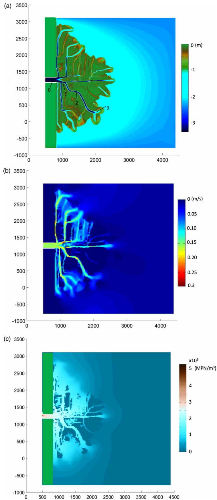
Figure 1 | (a) Bathymetry of the river delta. (b) Depth averaged velocity across the river delta for a river discharge of 100 \text{ m}^3/\text{s} . (c) E. coli concentration (MPN/m 3 ) for a discharge of 100 \text{ m}^3/\text{s} .
