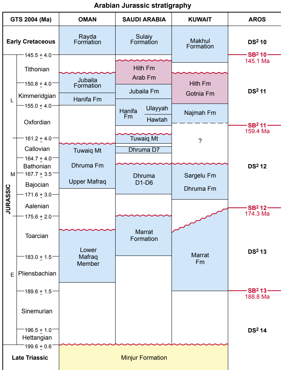
Figure 1: Correlation of Jurassic formations and hiatuses in Kuwait, Saudi Arabia and Oman. The ages of the Jurassic hiatuses are estimated by using biostratigraphic and Strontium-isotope data and the Geological Time Scale GTS 2004 (Gradstein et al., 2004). The Oman column is after Rousseau et al. (2006) except for the Tithonian and Berriasian, which is after Hughes Clark (1988). The Saudi Arabian column is after Enay et al. (1987), Le Nindre et al. (1990), Vaslet et al. (1991), Fischer et al. (2001) and D. Vaslet and Y.-M. Le Nindre (2006 written communications). The Kuwait column is after Al-Sahlan (2005) and A. Lomando (2006 written communication). The question mark in the Kuwait column indicates conflicting age interpretations for the Najmah Formation, which may extend to the Bathonian (G. Grabowski, 2006 written communication). The AROS (Arabian Orbital Stratigraphy) column indicates the orbital-forcing model second-order sequence boundaries (SB 2 ) and depositional sequences (DS 2 ).
