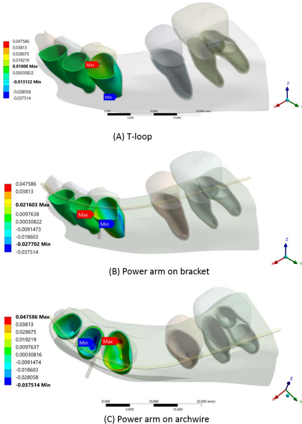
Figure 6. Comparison of the maximal (Max) and minimal (Min) dilatational stress in the PDL is shown for the three models: (A) TL, (B) PAB, and (C) PAW.
