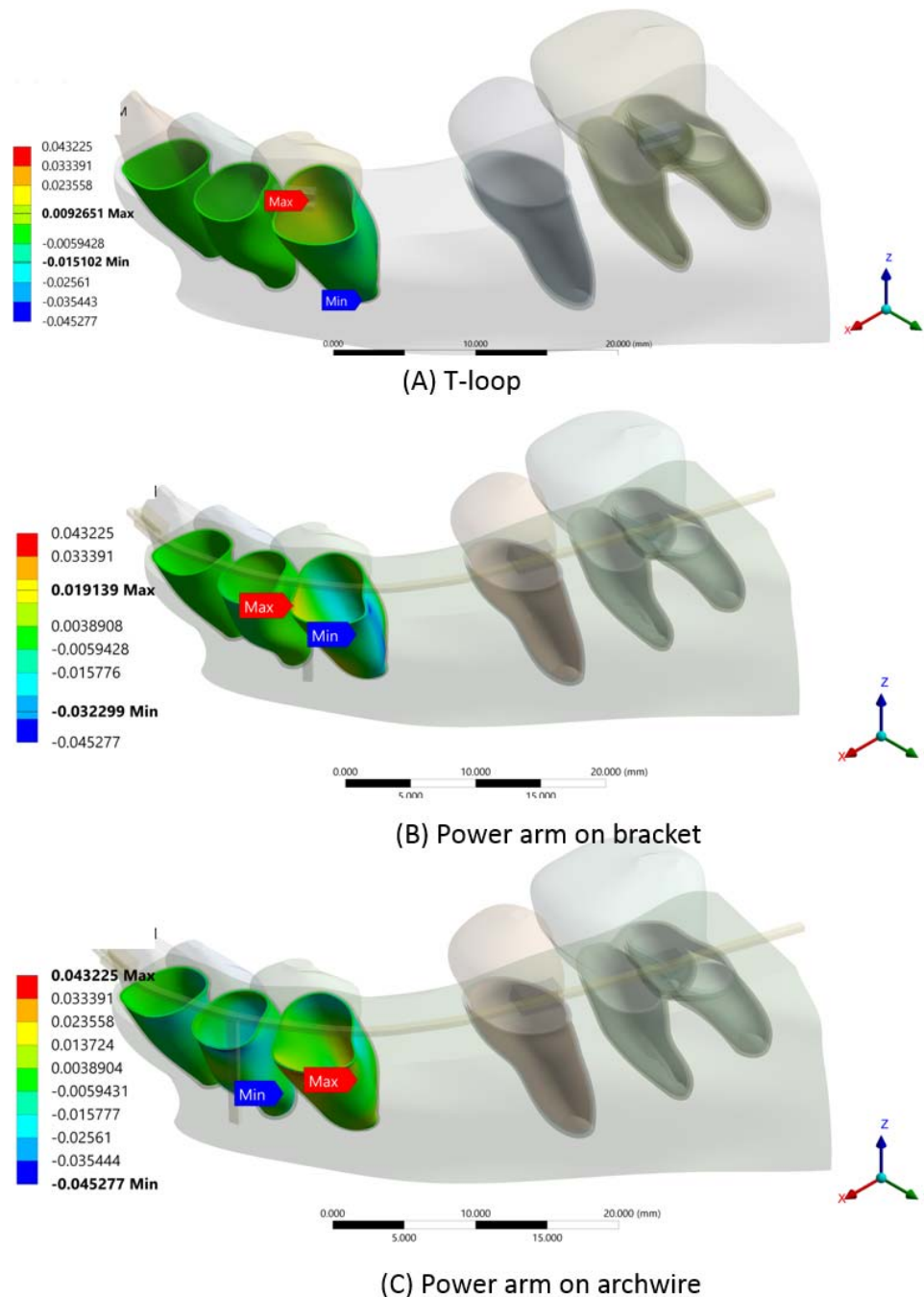
Figure 4. Comparison of the maximal (Max) and minimal (Min) third principal stress (P3) in the PDL is illustrated for the three models: (A) TL, (B) PAB, and (C) PAW. Positive stress is tensile and negative stress is in compression. See text for details.
