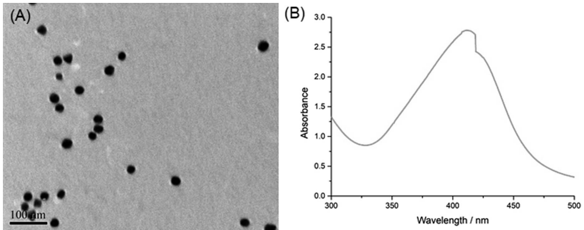
Figure 1. Characterization of NAg. (A) Typical TEM image of NAg. (B) UV-vis spectra of NAg.
