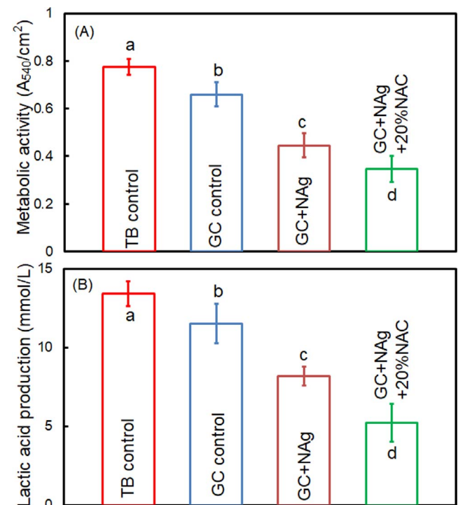
Figure 3. Quantitative antibacterial effects for biofilm grown on cement disks. (A) Metabolic activity. (B) Lactic acid production. The different letters indicate significant differences between groups ( P < .05 ).
