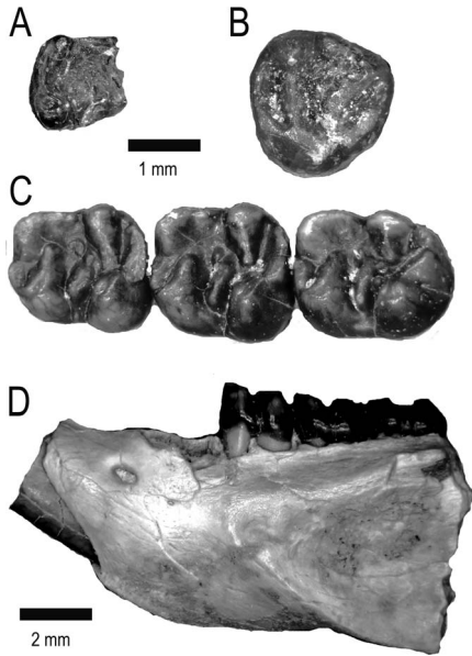
Fig. 2. Dentition and dentary of Mattimys and Tillomys from the Washakie Basin. A, Mattimys sp., FMNH PM 56559, right m1 (partial). B, ? T. senex , FMNH PM 1505, left M3. C–D, T. senex , FMNH PM 55908. C, left m1–m3, occlusal view. D, lateral view of dentary. A–C to same scale (above), D to different scale (below).
