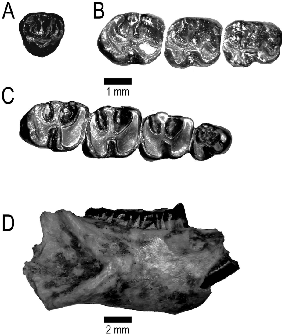
Fig. 4. Cheek teeth of Pareumys flynni from the Washakie Basin. A, FMNH PM 42080, right M3. B, FMNH PM 55121, right m1–m3. C–D, FMNH PM 55060 (holotype). C, right p4–m3, occlusal view. D, lateral view of dentary. Occlusal views all teeth to same scale (above), dentary to different scale (below).
