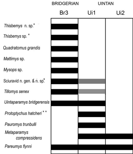
Fig. 5. Occurrence of rodent species throughout the Adobe Town Member of the Washakie Formation. Twk1: Lower (late Bridgerian, Br3); Twk2: Middle (early Uintan, Ui1); Twk3: Upper (middle Uintan, Ui2). Black bars = occurrence; gray bar = possible occurrence. *, species not yet described, **, species described by Turnbull (1991).
