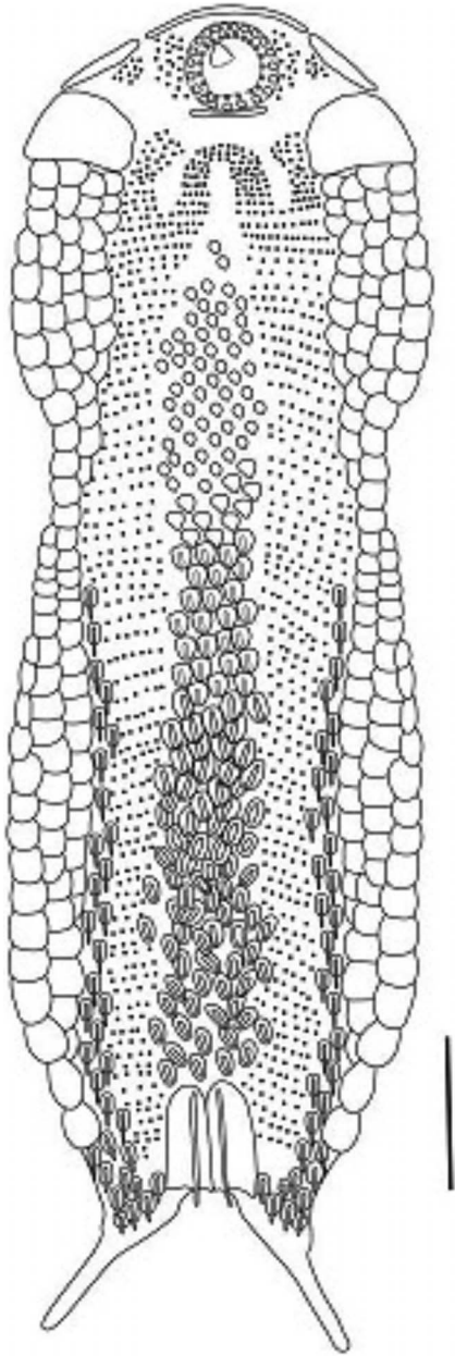
Fig. 3. Drawing of ventral aspect of Lepidodermella weissi holotype. Scale bar = 12 \mu m. The mouth is the round feature at the anterior end; a pharyngeal "tooth" is visible within the mouth. The cephalion is visible just anterior to the mouth. Epipleuria are lateral to the cephalion. The hypopleuria are the largest plates visible on the head. The hypostomion is a narrow, transverse element in contact with the posterior edge of the mouth. Patches of motor cilia (denoted as dots) are visible on either side of the mouth (longer sensory cilia are not shown but can be
