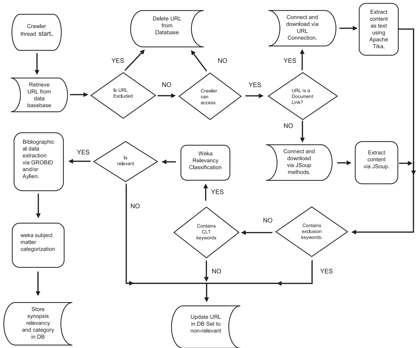
Figure 1.—Flowchart showing Uniform Resource Locator (URL) processing steps. DB = database; CLT = cross-laminated timber.
