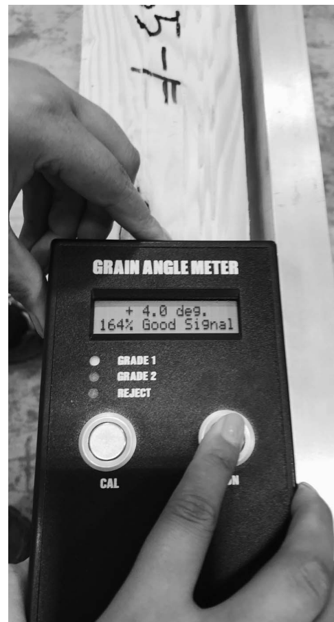
Figure 1.—Metriguard’s grain angle meter.
