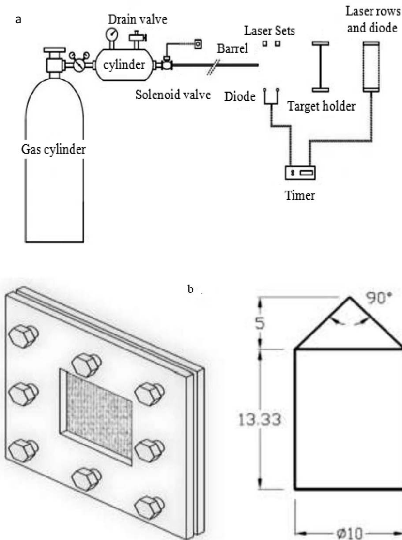
Figure 1.—Schematic representation of (a) the experimental setup for high-velocity impact tests (Pol et al. 2013), (b) sample holder (Mehrabani et al. 2016), and (c) projectile.
