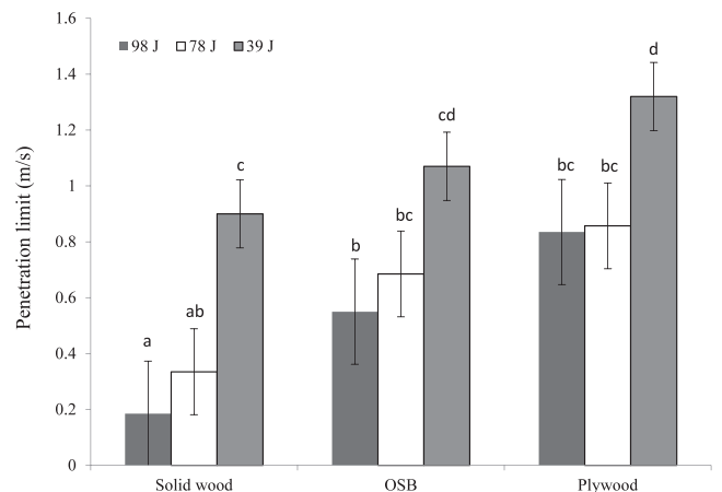
Figure 6.—Penetration limit of studied materials.
