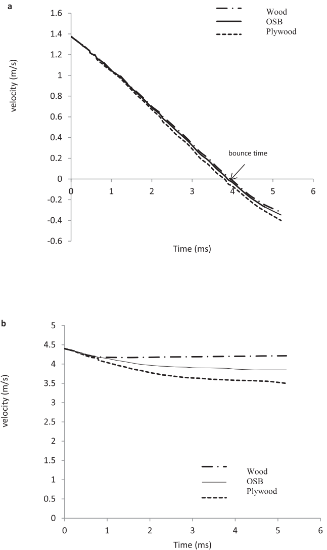
Figure 5.—Velocity-time response for materials subjected to (a) 10 J and (b) 98 J energy.
