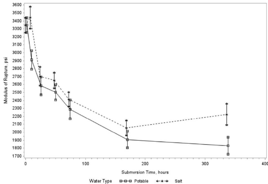
Figure 3.—Loss in modulus of rupture (MOR) of samples removed from full-size oriented strand board (OSB) panels as a function of submersion time in either potable or salt water. Each mean represents approximately 24 (parallel to strength axis) samples and consists of 3 brands and both interior and edge samples. Bars are offset slightly to allow better visibility.
