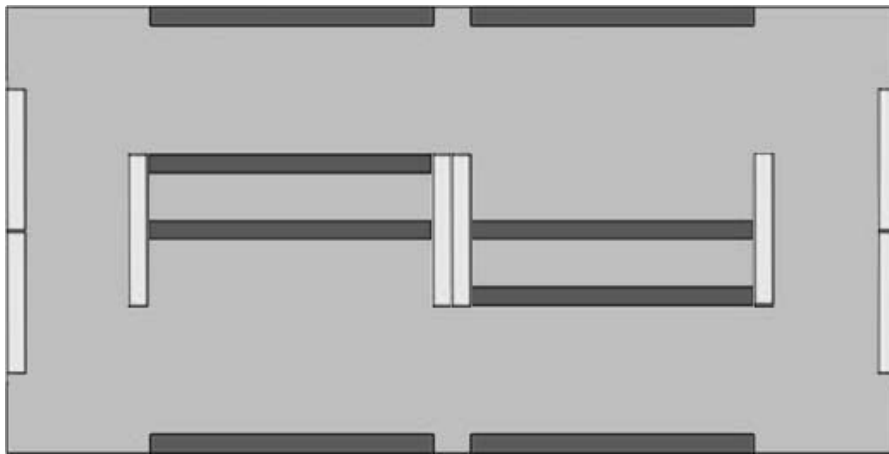
Figure 1.—Schematic diagram illustrating location of four types of samples removed from each panel (i.e., from the edge, the interior, parallel to the strength axis and perpendicular to the strength axis). A total of 16 samples were removed from each panel.
