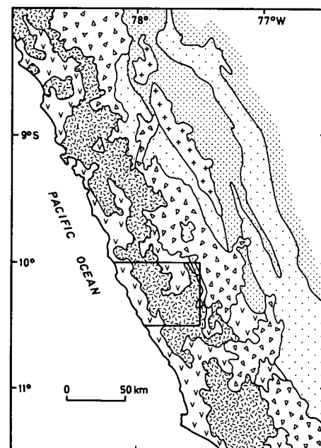
Figure 1. Map showing the extent of the Coastal Batholith of Peru (after Bellido and others, 1972) and locations of the area described and of section A–B of Figure 12.
