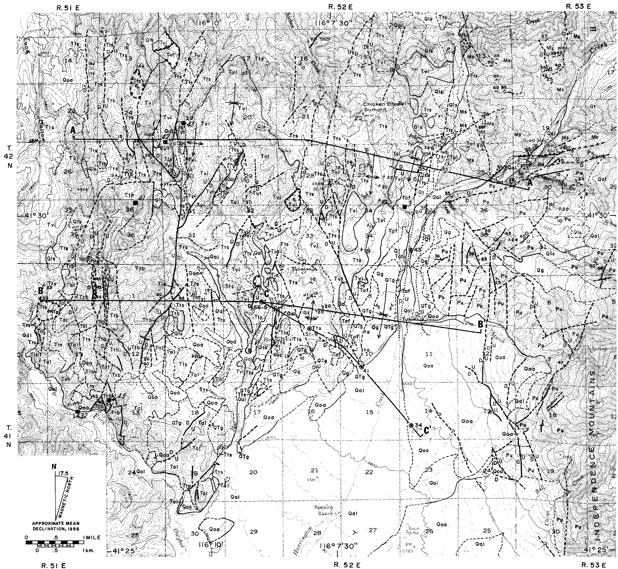
Figure 2. Geology of the Tuscarora geothermal area, Elko County, Nevada.
