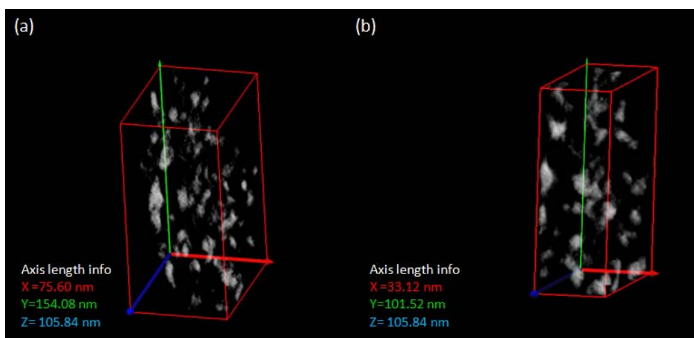
FIG. 5. — Three-dimensional TEM image of nanodiamond nanomatrix containing 25 w/w% nanodiamond concentration prepared with (a) 3.3 \times 10^{-4} mol/g-rubber TBHP/TEPA and (b) 6.6 \times 10^{-5} mol/g-rubber TBHP/TEPA.
