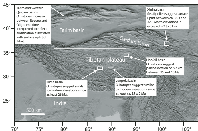
Figure 1. Shaded relief map of the Tibetan plateau and surrounding regions, showing localities of Eocene to Oligocene age basins that have yielded quantitative estimates of paleoelevation.
