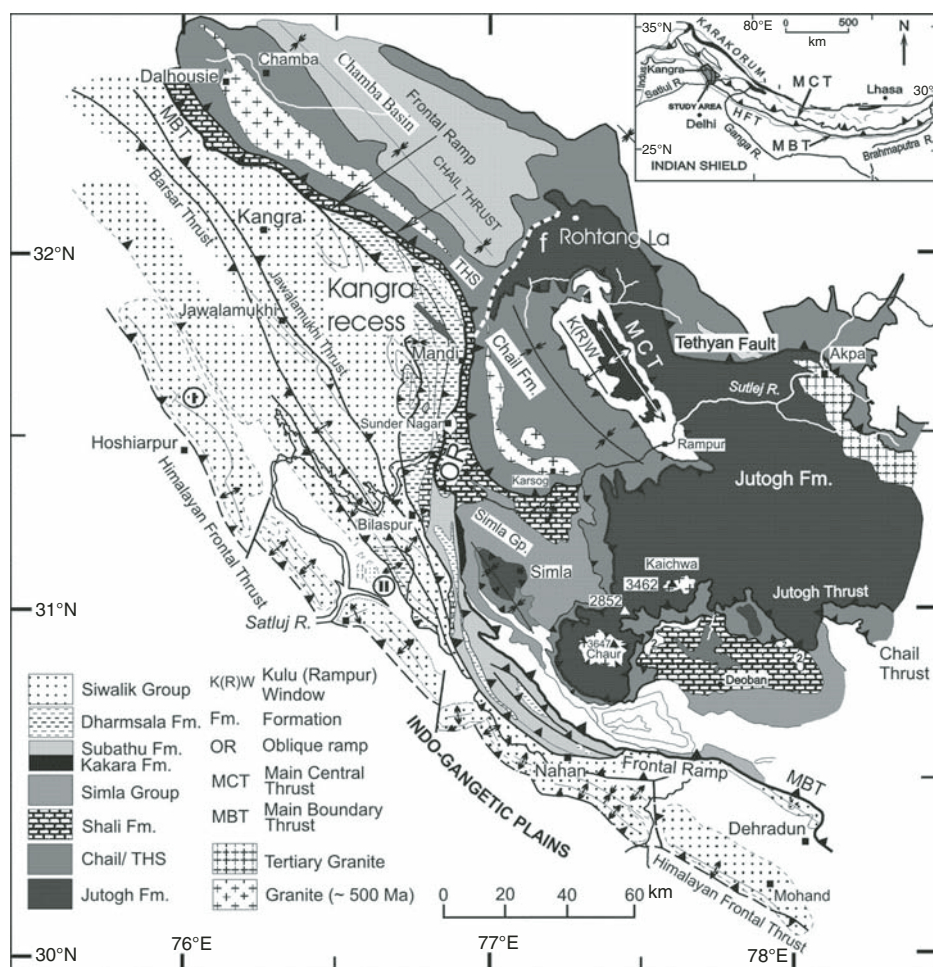
Figure 1. Geological map of a part of the Himachal Himalaya. The propagation and extension of the oblique ramp into the hanging wall, marking the boundary between the Chail Formation and the Tethys Himalayan sequence (THS), is shown by a white broken line. K(R)W—Kulu (Rampur) Window; Fm.—Formation; OR—Oblique ramp; MCT—Main Central Thrust; MBT—Main Boundary Thrust.
