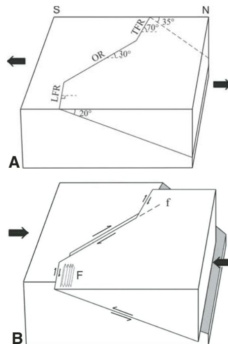
Figure 2. Simplified model showing two stages in the structural evolution of the Kangra recess. A: Geometry of initial fracture. LFR—leading frontal ramp; TFR—trailing frontal ramp; OR—oblique ramp; N-S—north and south directions. Note the variation of dip at the leading and trailing frontal ramps. B: Formation of folds (F), and extension of the oblique ramp fault (f) during the Himalayan orogeny.
