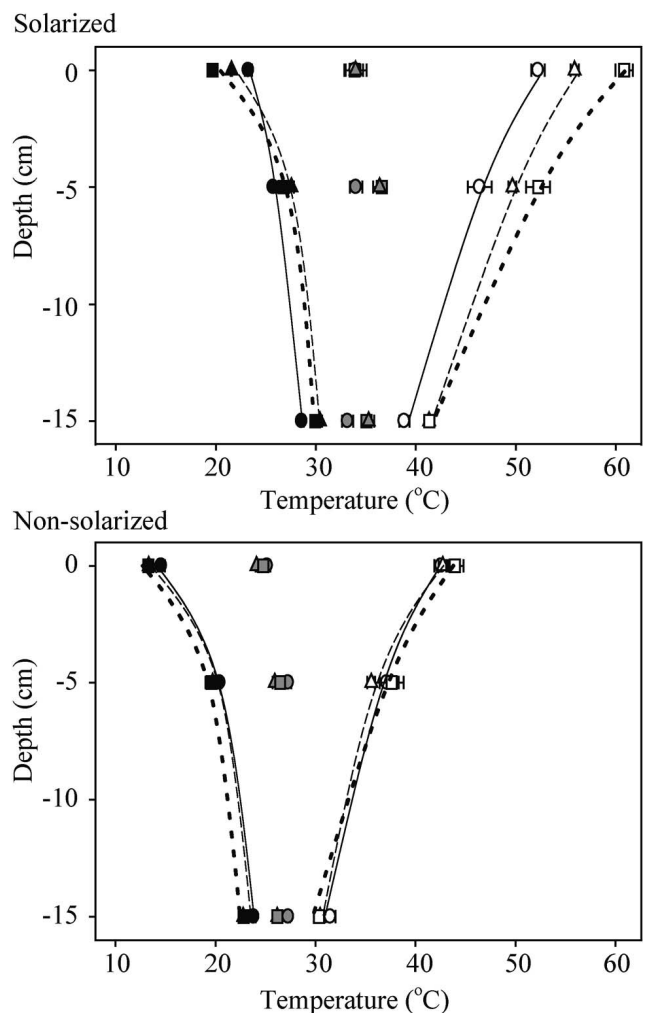
Fig. 3. The effect of different gravel thickness treatments (circle: 0 cm, triangle: 2.5 cm, square: 7.5 cm) on average maximum (open symbols), minimum (filled symbols), and mean average (gray symbols) daily temperature in different depths in solarized and non-solarized plots in trial 2 in CA. Non-linear regression lines are shown for each gravel treatment (solid lines: 0 cm gravel, dashed lines: 2.5 cm gravel, dotted lines: 7.5 cm gravel thickness). Similar trends were observed in other trials.
