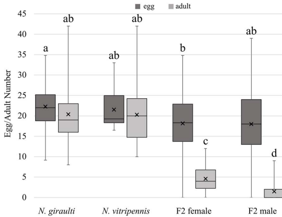
Fig. 1. Number of eggs/adults of each cross type. Boxes enclose the 25th to 75th percentiles and whiskers designate minimum and maximum values. The center horizontal line marks the median value and the X marks the mean value. Different letters over the boxes denote significant differences ( P < 0.05 ). Sample sizes: Nasonia giraulti = 35, N. vitripennis = 32, F 2 female = 66, F 2 male = 78.
