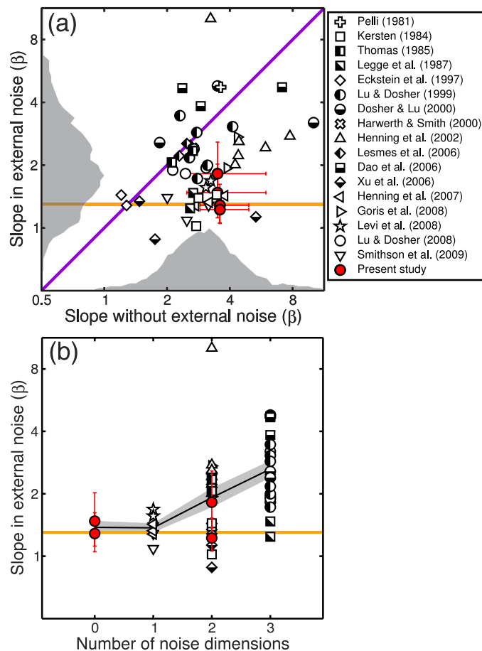
Figure 3. Slopes of the psychometric function (Weibull \beta ), with and without external noise, from 18 studies (Dao et al., 2006; Doshier & Lu, 2000; Eckstein et al., 1997; Goris et al., 2008; Harwerth & Smith, 2000; Henning et al., 2002; Henning & Wichmann, 2007; Kersten, 1984; Legge et al., 1987; Lesmes et al., 2006; Levi et al., 2008; Lu & Doshier, 1999, 2008; Pelli, 1981; Smithson et al., 2009; Thomas, 1985; Xu et al., 2006) on noise masking, including Experiment 1 here. Symbols indicate the study, as shown in the legend. (In some cases, it was necessary to extract data on proportion correct from published figures [using computer software] and fit them with Weibull functions to derive estimates of \beta ourselves.) The shaded areas in (a) are histograms showing the distributions of \beta values from the 18 studies (note that the peak of each of these is at \beta > 1.3 ). Panel (b) shows the ordinate data replotted as a function of the number of noise dimensions. Dynamic 2D noise, which varies in time, spatial frequency, and orientation, can be considered to have three dimensions. Lower dimensional noise varies in only a subset of these dimensions. The black curve and shaded region show the mean and \pm 1SE . Error bars on the red symbols are 95% confidence intervals obtained by bootstrap resampling.
