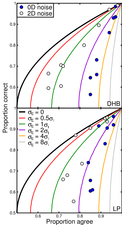
Figure 4. Double-pass consistency results (Experiment 2) for two observers (different panels) for 0D (blue symbols) and 2D (white symbols) noise masks. The curves are predictions (obtained by stochastic simulation [Klein & Levi, 2009]) of the noisy ideal observer model for different ratios of external:internal noise (given by the legend in the lower panel, where \sigma_E is external noise and \sigma_I is internal noise). The black curve ( \sigma_E = 0 ) is also the prediction of the gain control model and applies to all situations where there is no external noise (e.g., baseline detection thresholds) (Klein & Levi, 2009).
