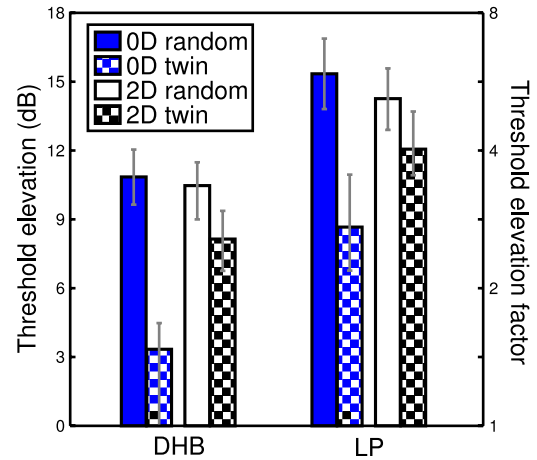
Figure 5. Random and twin noise configuration results (Experiment 3) for two observers (left and right). Bars show threshold elevation for 0D and 2D noise masks using each type of noise configuration (see legend). Empirical thresholds were determined using the method of constant stimuli with 1,800 trials per condition. The noisy ideal observer model predicts that threshold elevation should be 0 dB for the twin conditions (checked bars). The gain control model predicts that the level of masking should be the same for the random and twin conditions. Deviations from these predictions are discussed in the main text. Error bars show bootstrapped 95% confidence intervals.
