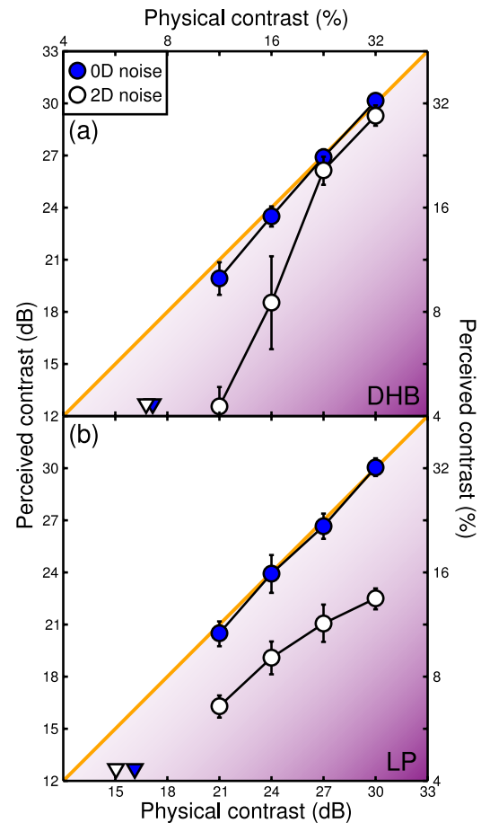
Figure 6. Perceived contrast in noise (Experiment 4) for two observers (top and bottom). The physical target contrast is plotted along the abscissa and the perceived (matching) contrast along the ordinate. If a mask had no effect on perceived contrast, the results should fall on the diagonal orange line. Results falling below this line (in the purple graded shading) indicate that perceived contrast was attenuated by the mask with darker shading corresponding to stronger attenuation. Error bars show 95% confidence intervals obtained by bootstrap resampling. Triangles placed on the x-axis indicate (masked) contrast detection thresholds for each condition for the same mask contrast as was used in the matching one.
