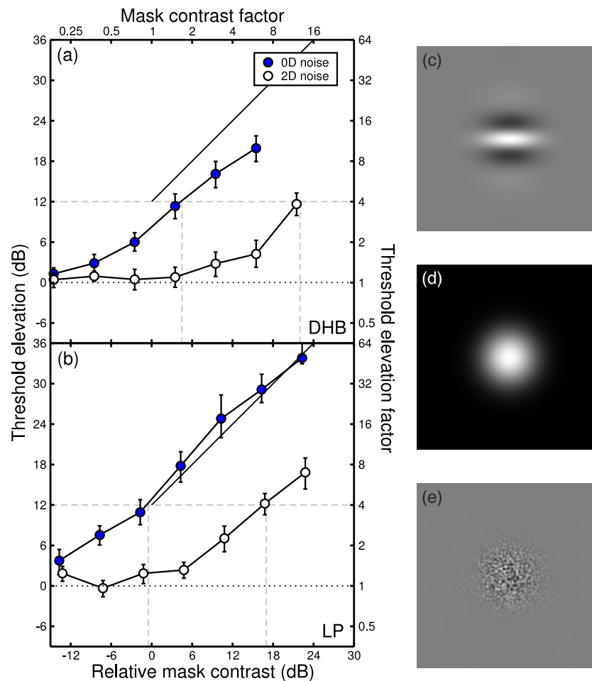
Figure 2. Noise-masking results (preliminary experiment) for two observers (top and bottom) and example stimuli. (a, b) Results are plotted as functions of relative mask contrast (e.g., they are scaled by the detection thresholds for the masks). The diagonal lines have unit slope for reference, and error bars give 95% confidence intervals obtained by bootstrap resampling. The intersections of the horizontal and vertical dashed lines indicate the mask contrasts that produced equal levels of threshold elevation (12 dB), used in subsequent experiments. (c) Log-Gabor target. (d) The Gaussian envelope used to window the noise (see Methods ). (e) An example of windowed 2D white noise.
