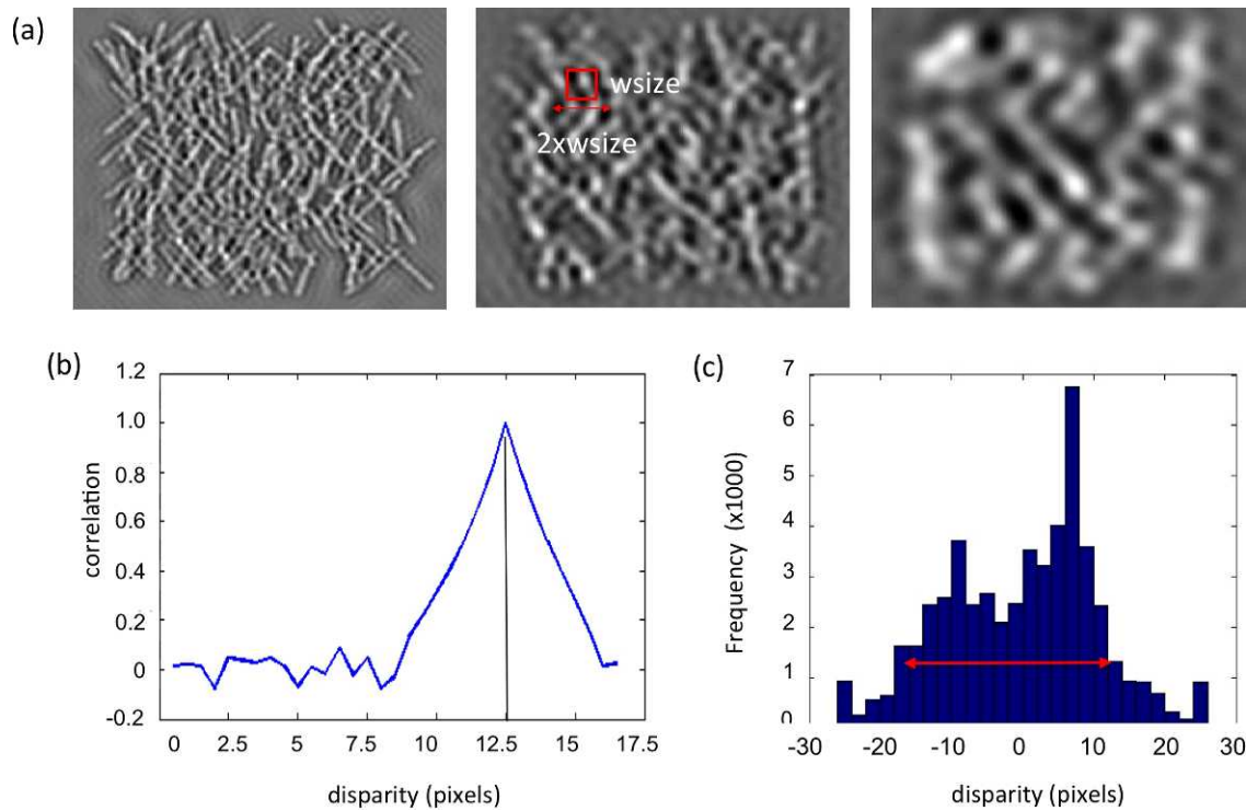
Figure 5. (a) Diagram illustrates three levels of prefiltering of the image before cross-correlation at a specific scale. Red square illustrates an example correlation window and range. (b) Correlation as a function of disparity. The peak of the function is chosen as the disparity. (c) Histogram showing frequency of extracted disparities for all image locations. The standard deviation of the distribution is chosen as a measure of thickness of the volume of elements.
