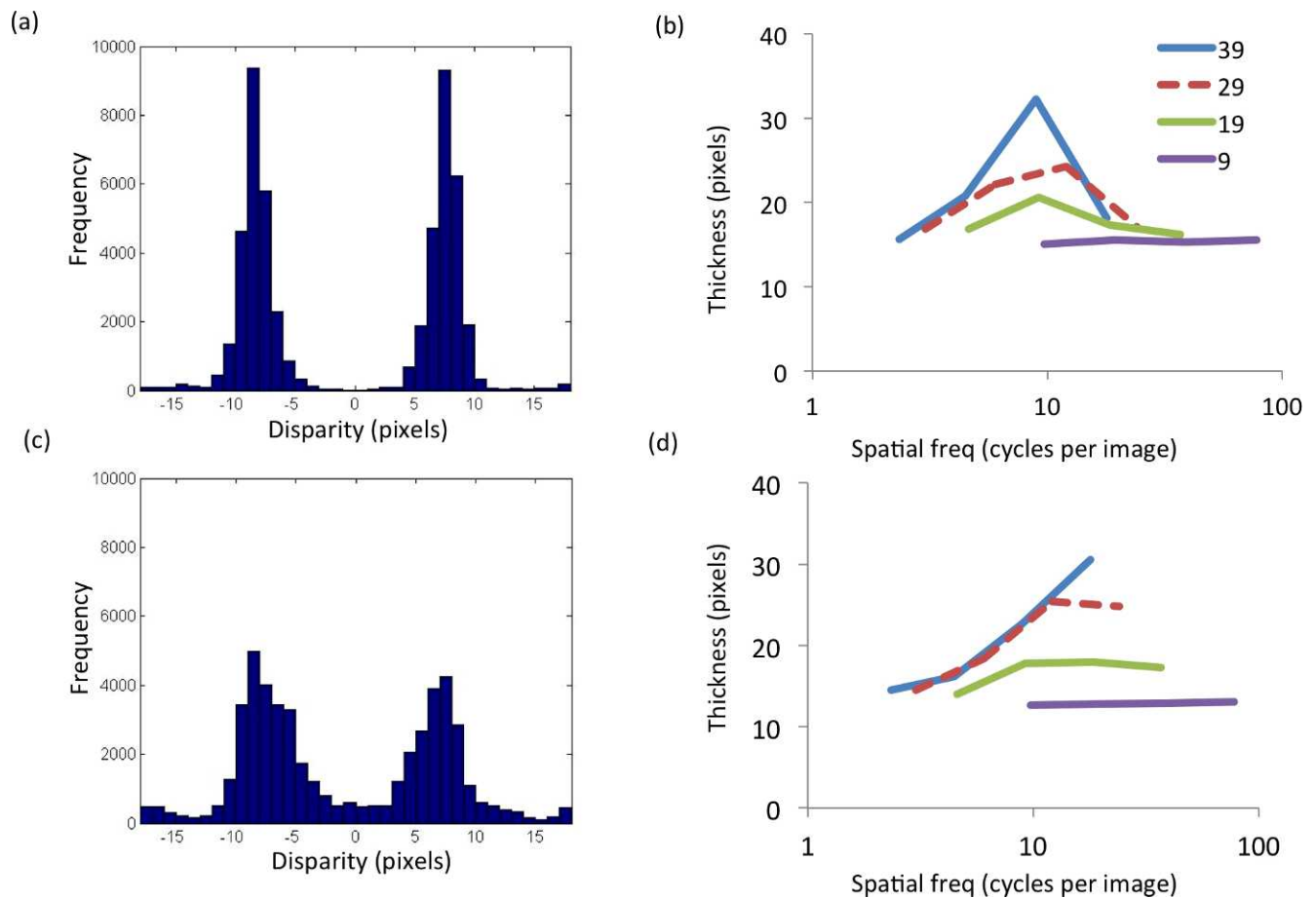
Figure 6. (a) Frequency of extracted disparities for planes stimulus, for f=1/w relationship, and a correlation window size of 19 pixels. (b) Extracted thickness of the disparity distribution for plane stimulus as a function of spatial frequency (cycles per image) for four window sizes. (c) Frequency of extracted disparities for volume stimulus, same parameters as in (a). (d) Extracted thickness of disparity distribution for volume stimulus.
