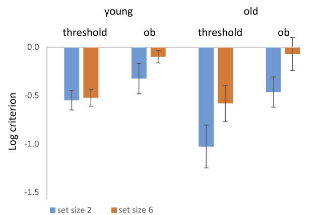
Figure 4. Log criterion. threshold = threshold contrast; ob = octave-below threshold contrast. Error bars represent standard errors of the mean.
