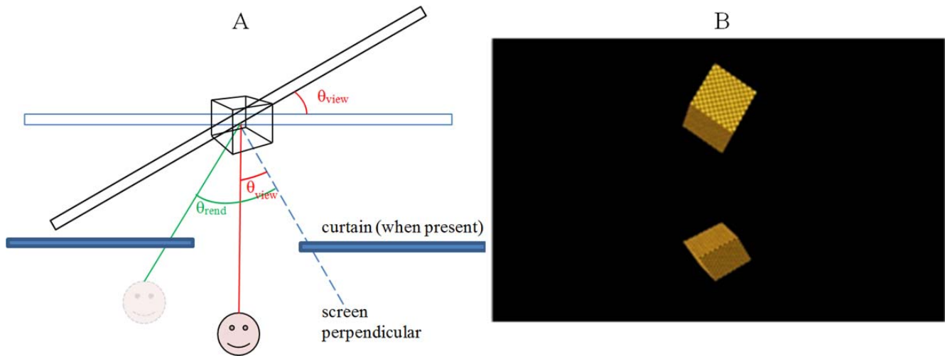
Figure 2. Experimental setup seen from above (A) and example stimulus (B). (A) The heads of two possible viewers are sketched. The head drawn with solid lines represents the actual position of the participant, whose line of sight to the screen (red line) is at angle \theta_{\text{view}} to the perpendicular (blue dashed line). The head drawn with dotted lines represents the position of a hypothetical viewer whose line of sight is at \theta_{\text{rend}} (green line). The obliquely rendered cube is projected correctly for this hypothetical viewer. It is correct for the participant only when \theta_{\text{view}} = \theta_{\text{rend}} . The normal-rendered cube is projected correctly for a second hypothetical viewer whose line of sight is perpendicular to the screen. In some blocks, a curtain was pulled across so as to occlude the edges of the screen from the participant's view. (B) Stimulus drawn on the display screen. Here, the top cube is the normal-rendered cube (rendered for viewing perpendicular to the screen) and the bottom cube is the obliquely rendered cube, here rendered for a viewing angle of 45^\circ . You may find that the bottom cube appears less distorted when viewed from 45^\circ to the right.
