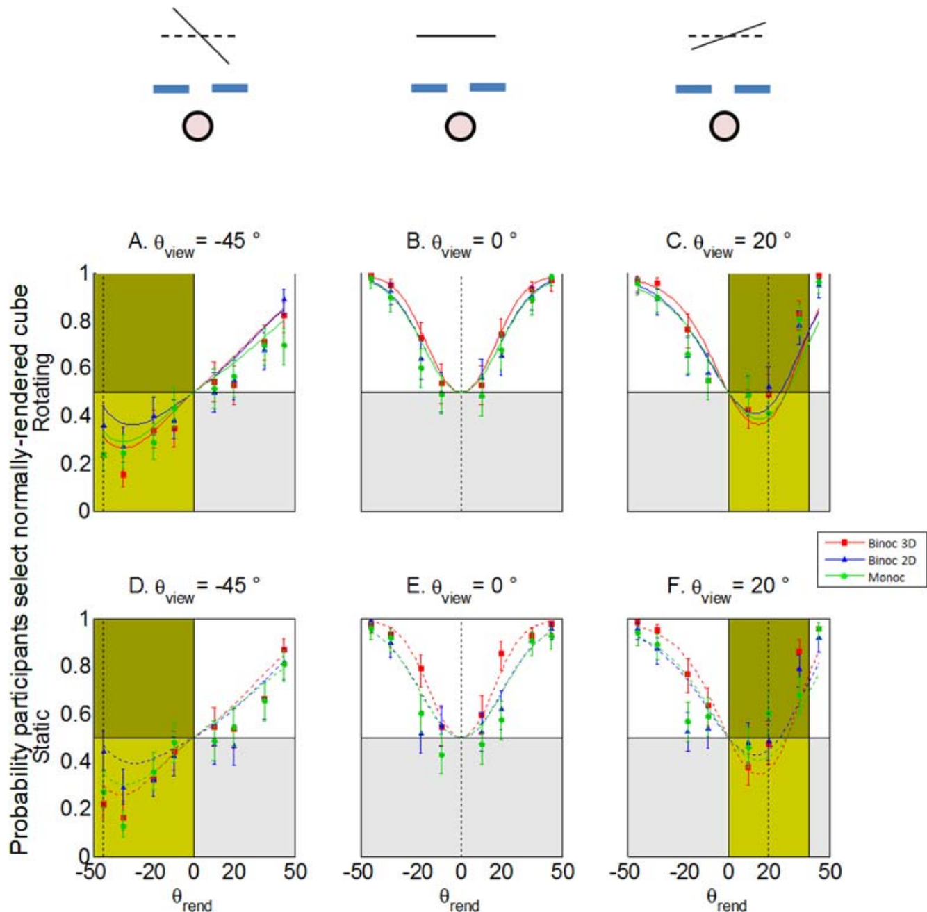
Figure 6. Results from the frame-occluded condition. As for Figure 5, except here a curtain prevented the subjects from seeing the edges of the screen.
