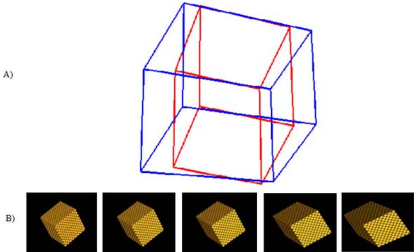
Figure 3. (A) Rendered image on-screen for two different render angles. The two cubes are projections from exactly the same virtual cube in space, but the red cube is rendered for perpendicular viewing, while the blue cube is rendered for a viewing angle of 45^\circ . If you view the image with one eye from 45^\circ to the right, the blue cube should appear as the red cube does when viewed normally. (B) Example cube rendered for five different angles used in our experiments. From left to right, \theta_{\text{rend}} = 0^\circ, 10^\circ, 20^\circ, 35^\circ, and 45^\circ .
