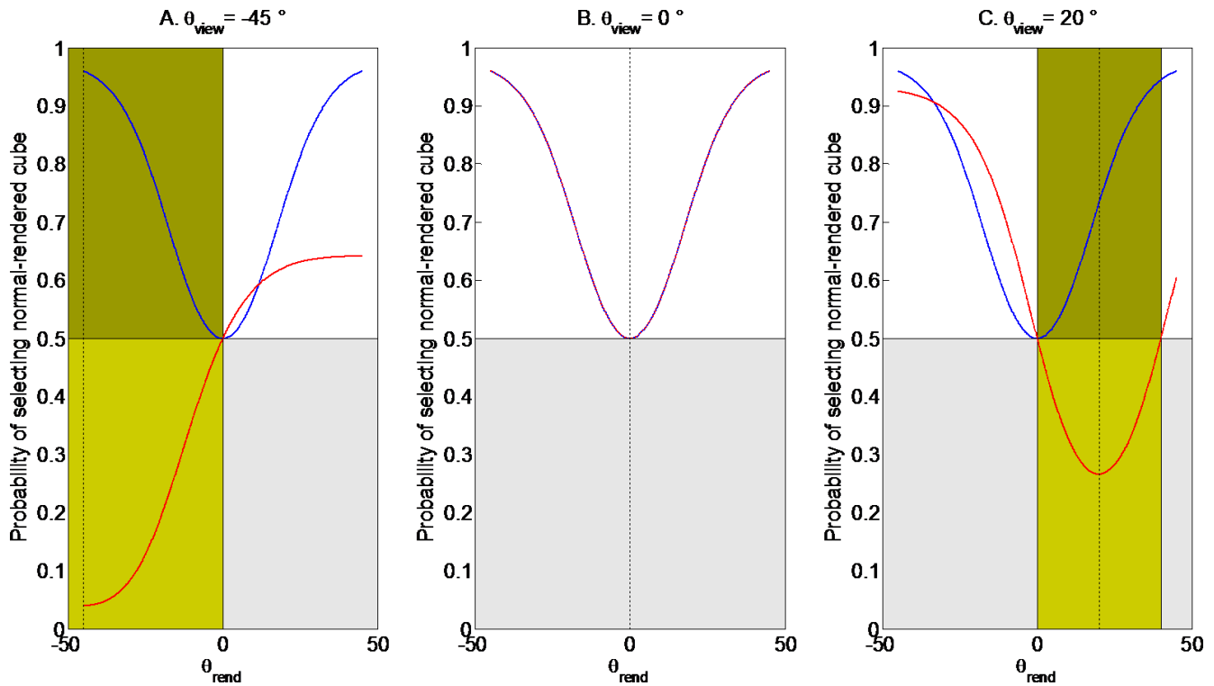
Figure 4. Model predictions with perfect compensation for oblique viewing (blue) and no compensation (red). Curves show the probability that the model selects the normal-rendered cube as being more veridical, plotted as a function of render angle \theta_{\text{rend}} for three different viewing angles \theta_{\text{view}} . Model parameters were r = s = 24^\circ ; for the blue curves, A = 3 and B = 0 (perfect compensation for oblique viewing); for the red curves, A = 0 and B = 3 (no compensation). White and gray regions show where the normal-rendered cube is also closer to geometrically correct than the oblique cube ( |\theta_{\text{rend}} - \theta_{\text{view}}| > |\theta_{\text{view}}| ); yellow-shaded regions show where the obliquely rendered cube is closer to geometrically correct ( |\theta_{\text{rend}} - \theta_{\text{view}}| < |\theta_{\text{view}}| ). Light shading (white or light yellow) is used to show the direction of preference expected under the no-compensation model, i.e., below 0.5 where |\theta_{\text{rend}} - \theta_{\text{view}}| < |\theta_{\text{view}}| and above 0.5 otherwise.
