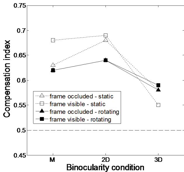
Figure 7. Compensation index C , defined as the ratio A/(A + B) . A and B are model parameters modeling the strength of the preference for normal rendering and for geometrical correctness, respectively. Higher values of C indicate more compensation for oblique viewing. The dashed horizontal line marks where both weights are equal. This figure shows the values derived from fits to data pooled across all subjects. To carry out the analysis of significance, we derived compensation indices for individual subjects from fits pooled to data from that subject only.
