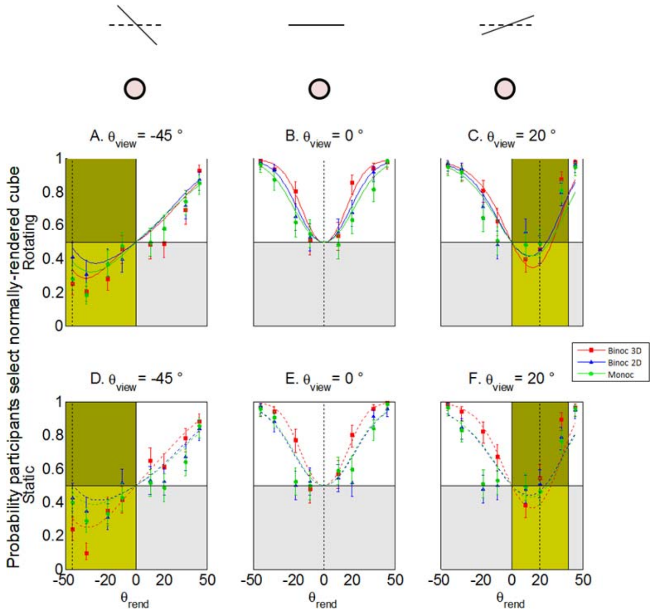
Figure 5. Results from the frame-visible condition. The vertical axis displays the proportion of trials on which subjects reported the normal-rendered cube as appearing “more cube-like.” Results are plotted as a function of \theta_{\text{rend}} , the viewing angle for which the obliquely rendered cube was drawn. Subjects would therefore necessarily be at chance at \theta_{\text{rend}} = 0 . Data were pooled across subjects; each data point represents 176 trials from 11 subjects. Error bars show 95% confidence intervals using simple binomial statistics. The top row (solid lines, figures A, B, C) is for trials with rotating cubes, the bottom row (dashed lines, figures D, E, F) is for trials with static cubes. Figures A and D show data from \theta_{\text{view}} = -45^\circ , figures B and E from \theta_{\text{view}} = 0^\circ , and figures C and F from \theta_{\text{view}} = 20^\circ . Shading as in Figure 4.
