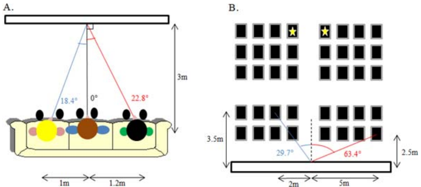
Figure 1. (A) A diagram to illustrate how viewing angles can change. If three people sit in the home watching television together, 3 m away from the screen and between 1 and 1.2 m apart, the viewing angle can be up to 23°. Angles are measured from perpendicular viewing (here we show a top-down diagram). (B) Viewing angles for different seats in a hypothetical cinema theater auditorium. Stars indicate the seats with viewing angles closest to ideal ( 0^\circ = frontoparallel).
