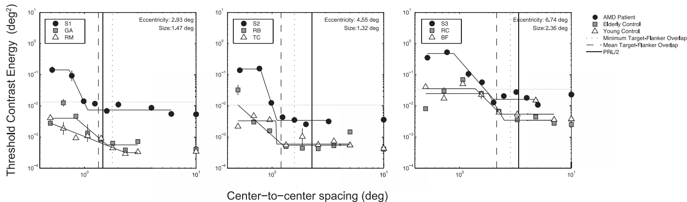
Figure 3. Threshold contrast energy as a function of center-to-center spacing. Each plot contains the data for an AMD participant and the two controls tested at the same retinal location as the AMD participant’s PRL. The dotted and dashed vertical lines delineate the minimum and mean target–flanker spacings, respectively, when the target and flanker overlap. The solid vertical line specifies half the distance to the PRL (Bouma’s scaling factor of 0.5). The dotted horizontal lines indicate the contrast energy of the flanker. The data points on the far y-axis are contrast threshold for single target objects in the absence of flankers (baseline performance). The target eccentricity and size for each AMD participant and the paired controls are specified in the upper right of each plot.
