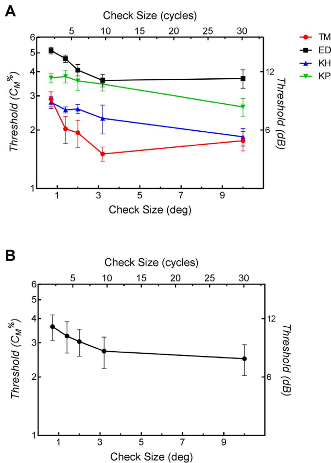
Figure 4. Contrast increment thresholds for each of the checked Battenberg stimuli and the full stimulus condition are shown for each observer (A) and the average of all four observers (B). The size of the check is represented as a function of degrees on the lower x axis, and number of cycles on the upper x axis. All error bars represent 1 SEM .
