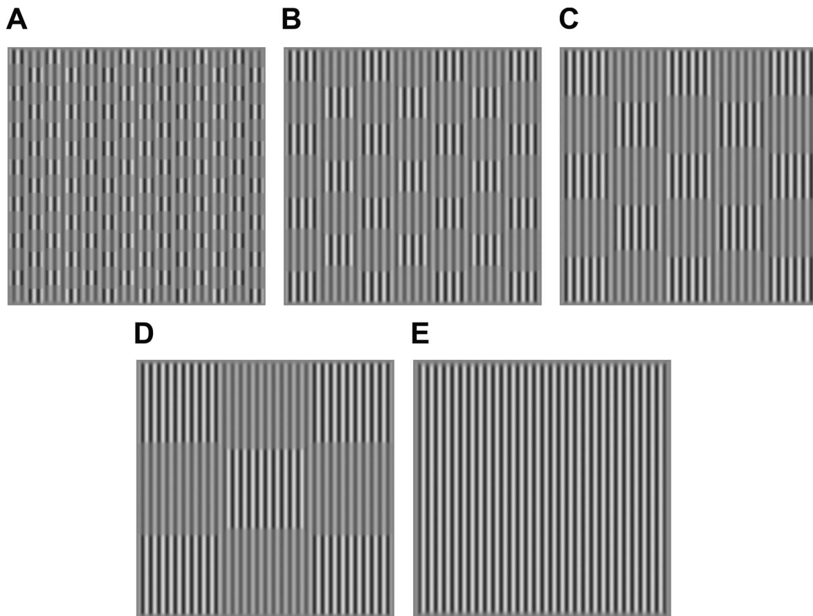
Figure 2. Examples of the stimuli used as the target stimulus in this experiment. Battenberg patterns which had check sizes of 0.71^\circ , 1.43^\circ , 2.00^\circ , or 3.33^\circ (A–D, respectively) were added to a full grating contrast pedestal ( 10^\circ side length). Panel E shows the target used in the full stimulus condition which was a full grating contrast increment added to a full grating pedestal.
