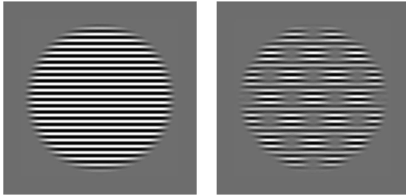
Figure 1. An example of the Swiss Cheese stimulus (right) and full stimulus (left) used in Meese and Summers (2007).
