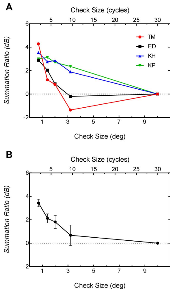
Figure 5. Raw thresholds are converted into summation ratios (Battenberg/Full) which represent the level of summation for each Battenberg stimulus. Ratios for the individual observers are shown in Panel A, and the group average is shown in Panel B. The size of the check is represented as a function of degrees on the lower x axis, and number of cycles on the upper x axis. Error bars represent 1 SEM .
