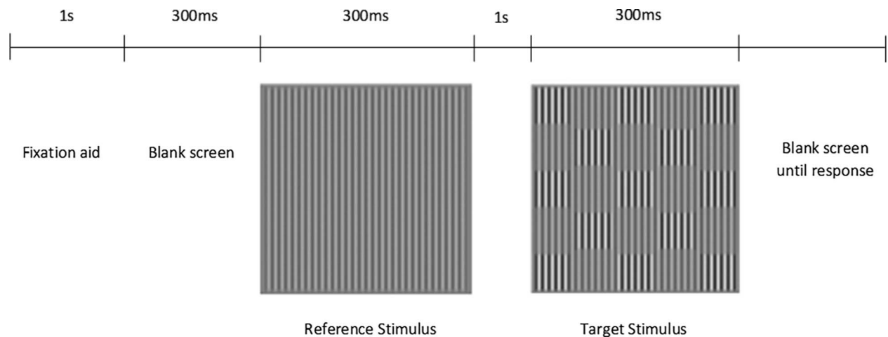
Figure 3. A schematic representation of a single trial. The trial began with a fixation point (1 s) followed by a blank screen set at mean luminance (300 ms). The stimulus intervals containing either the pedestal alone (reference) or the pedestal plus the contrast increment (target) were presented in a randomly selected order for 300 ms each, separated by a 1 s interstimulus interval set at mean luminance. A blank screen set at mean luminance was displayed until the observer made a response and remained for 1 s until the start of the next trial.
