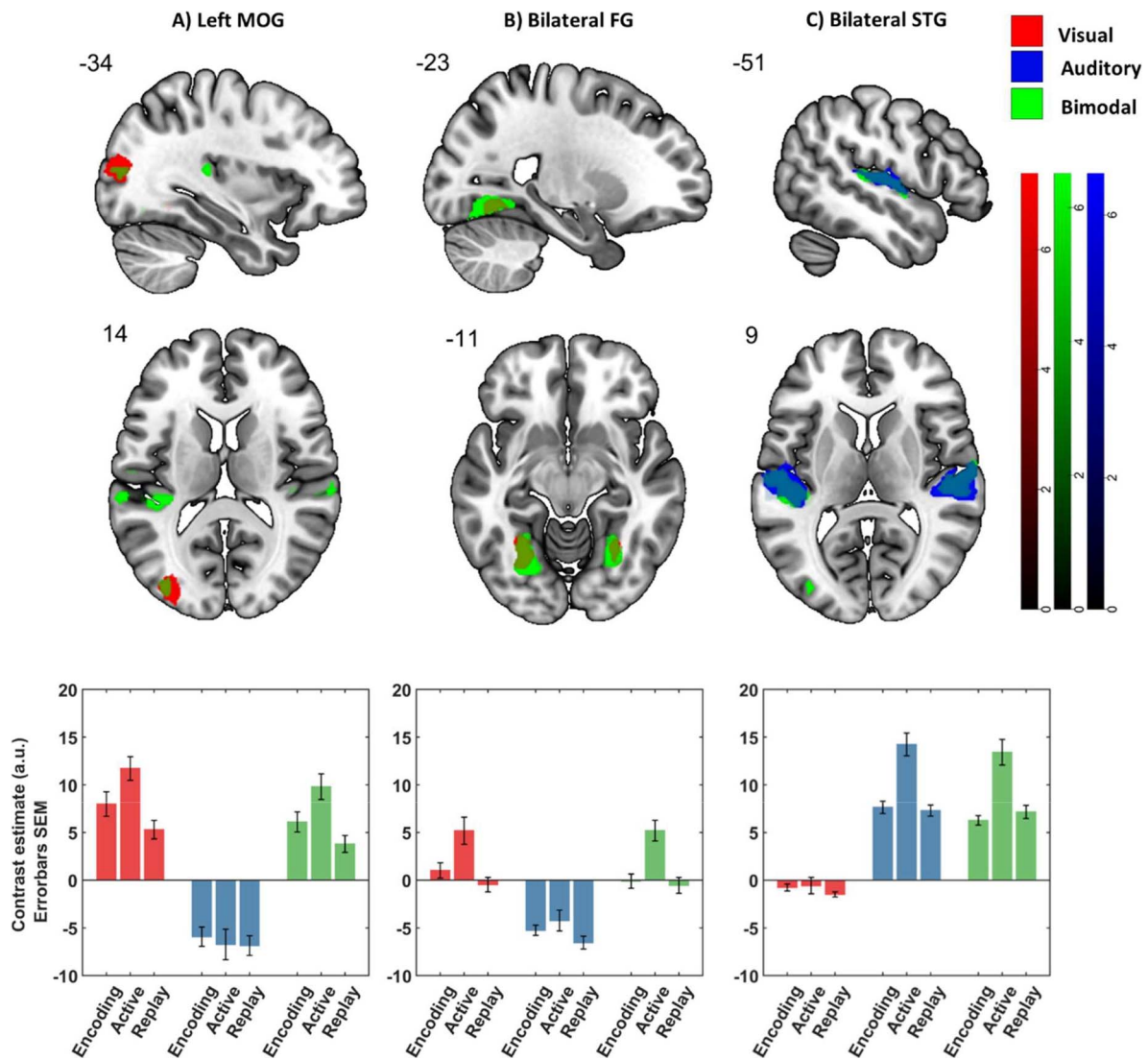
Figure 2. BOLD-enhanced areas from the conjunction contrast active > replay \cap active > motor control. The panels above depict BOLD enhancement for the different stimulus modalities and corresponding contrast estimates as retrieved from the respective clusters. (A) An area in the left middle occipital gyrus displayed enhancement, both in visual and bimodal stimulation. Contrast estimates reveal an increased activity for the encoding condition and a highly elevated enhancement for the active condition relative to the replay condition in the visual and bimodal modalities. No action-related modulation was observed in the auditory modality. (B) Bilateral enhancement in the fusiform gyrus (FG) for visual and bimodal stimulation. The encoding and replay conditions did not induce a BOLD enhancement in the FG cluster as the active condition. (C) The superior temporal gyrus was enhanced specifically in the auditory and bimodal condition. Top row, sagittal view; bottom row, axial view. Visual stimulation in red, auditory in blue, and bimodal in green. Color bars indicate T-scores. Threshold at 0.05 FWE.
