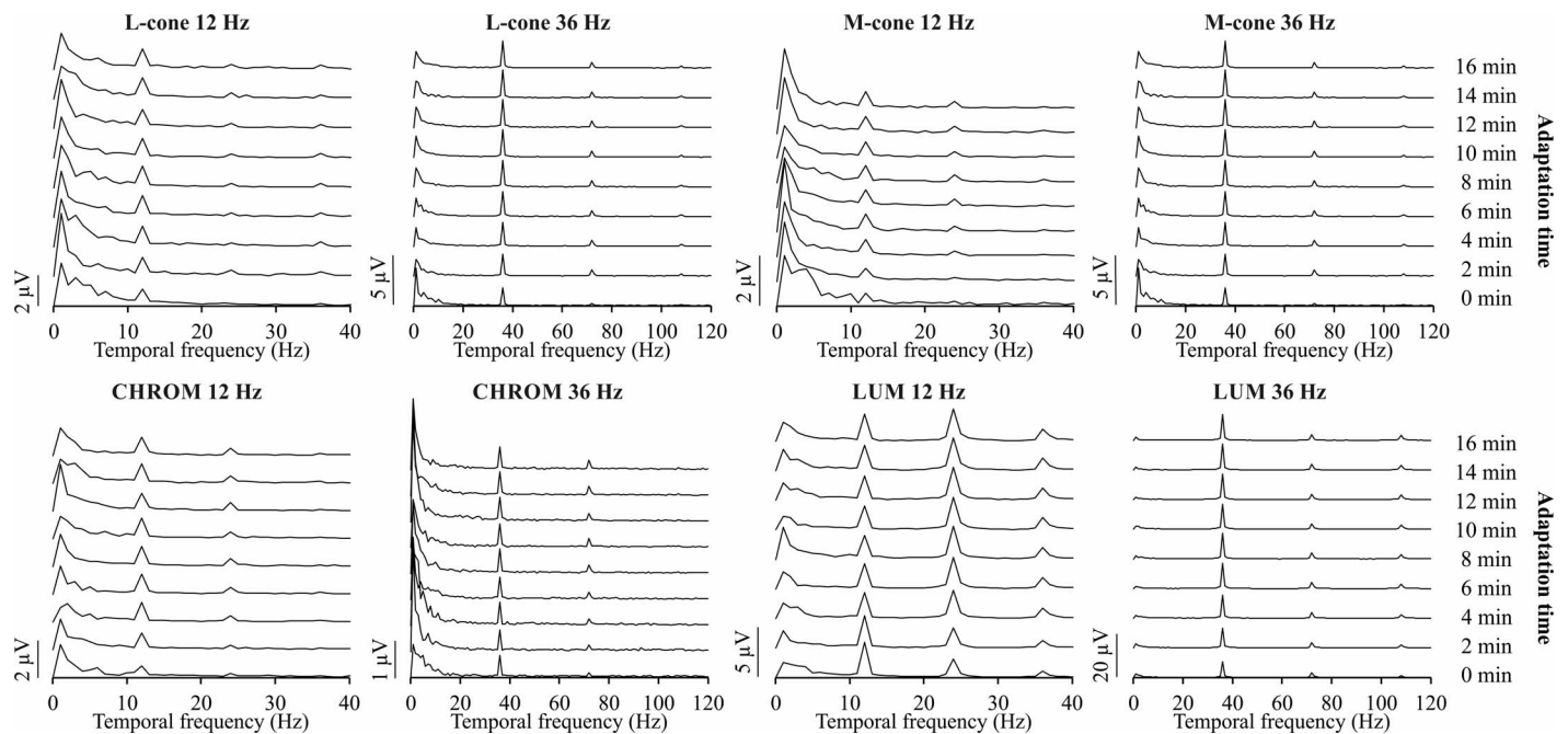
Figure 2. The amplitude as a function of temporal frequency of the group-averaged ERG responses for the eight stimulation conditions plotted separately for the different time points after light onset (given at far right). L-cone = L-cone isolating stimulus; M-cone = M-cone isolating stimulus; CHROM = chromatic stimulus; LUM = luminance stimulus.
