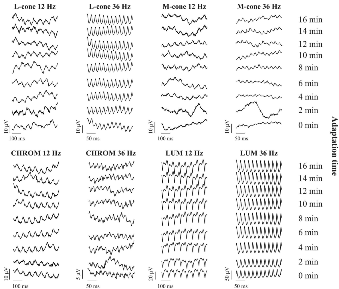
Figure 1. Group-averaged ERG traces for each stimulus condition during 16 min of light adaptation. Time points of each measurement are given on the far right. L-cone = L-cone isolating stimulus; M-cone = M-cone isolating stimulus; CHROM = chromatic stimulus; LUM = luminance stimulus.
