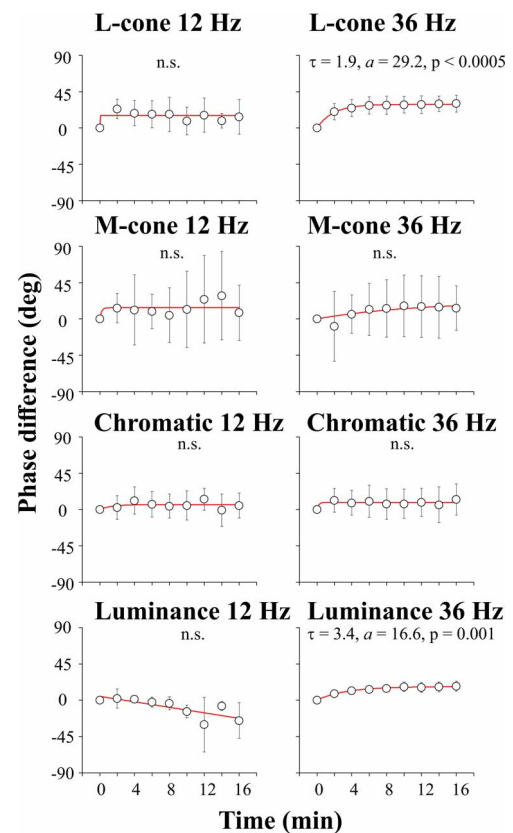
Figure 4. Averaged ( \pm SD ) phase shifts of the fundamental component (F) compared to the phase at t = 0 as a function of adaptation time for the eight different stimulus conditions. The data are presented in a similar manner as in Figure 3.
