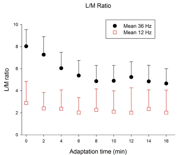
Figure 6. Mean L/M cone ERG amplitude ratio of the F components as a function of adaptation time obtained with 12- and 36-Hz L- and M-cone isolating stimuli. The ratios from 12-Hz data did not change during the adaptation period and did not differ strongly from unity, suggesting cone-opponent processing. The ratios obtained from the 36-Hz ERGs were larger, suggesting a luminance input. Interestingly, the ratios at 36-Hz decreased during light adaptation.
