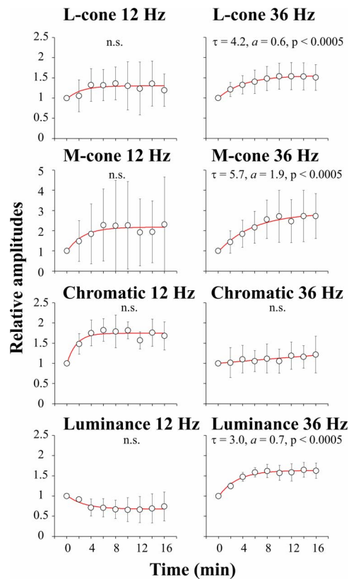
Figure 3. Averaged ( \pm SD ) normalized amplitude changes of the fundamental component (F) normalized to the amplitude at t = 0 as a function of adaptation time for the eight different stimulus conditions. The curves are fits of the data with Equation 2. P values are given for significant changes. Not significant = n.s. The estimates of a and \tau are displayed for the conditions with significant changes.
