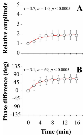
Figure 5. Averaged ( \pm SD ) normalized amplitude changes (A) and phase shifts (B) of the second harmonic component (2F) compared to the amplitude and phase at t = 0 as a function of adaptation time for the 12-Hz luminance stimulus. The data are presented in a similar manner as in Figure 3.
