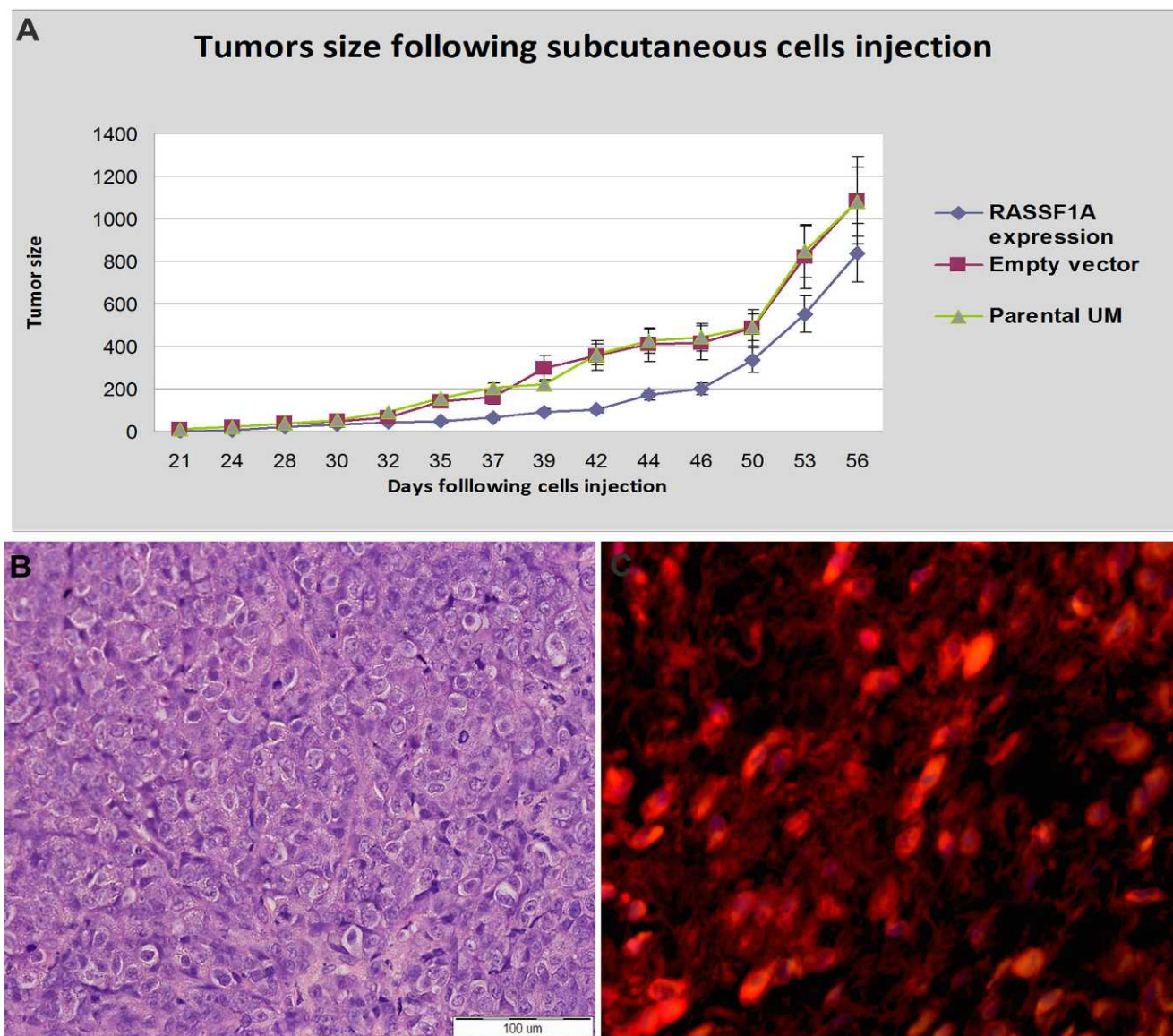
FIGURE 5. Subcutaneous tumor size (mm) following injection of 3 cell lines: RASSF1A -expressing cells, cells transfected with empty vector, and original UM-15. (A) All mice injected subcutaneously had tumors ( n = 17 ). Tumors were detected by day 28 in all mice injected with empty vector ( n = 6 ), by day 32 in mice injected with parental UM ( n = 6 ), and by day 39 in mice injected with RASSF1A -expressing cell line ( n = 5 ). Tumor growth was slower in mice injected with RASSF1A -expressing cells than in the other groups (NS). (B) Histologic findings of melanoma epithelioid cells with a low mitotic index from a subcutaneous tumor originated from original (non RASSF1A -expressing) UM cells. (C) RASSF1A positive immunostaining of subcutaneous tumor originated from RASSF1A -expressing UM cells ( n = 2 , red, \times 40 ).
