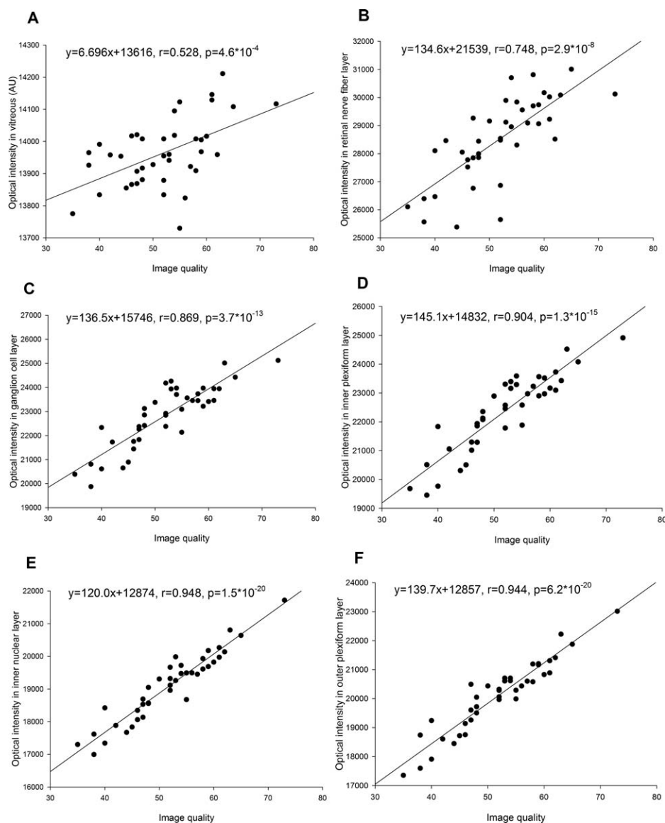
FIGURE 4. (A-F) Correlation of optical intensities in all retinal layers with image quality.
