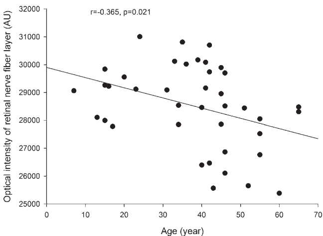
FIGURE 5. Correlation of optical intensity in retinal nerve fiber layer with age.
