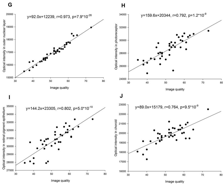
FIGURE 4. (G–J) Correlation of optical intensities in all retinal layers with image quality.
