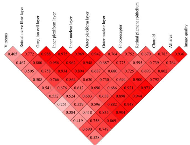
FIGURE 3. Correlation coefficient matrix of optical intensities among all layers and image quality. The numbers in each cell are the correlation coefficients.
