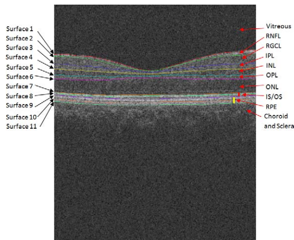
FIGURE 1. Segmented surfaces and regions on macular spectral-domain optical coherence tomography.
