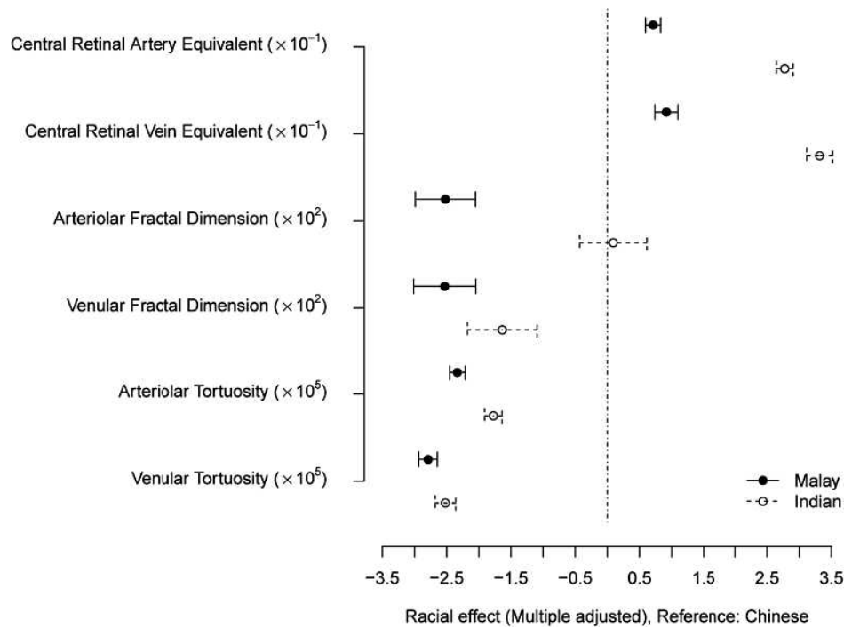
FIGURE 1. Racial difference of retinal vascular parameters, adjusting for age, sex, body mass index, systolic blood pressure, cholesterol, and glucose. The data presented are mean and SEs. Chinese serve as “reference,” and the racial effect is represented as the difference between Chinese and two other ethnic groups. Some numbers were multiplied by 10, to be shown in one graph regardless of the parameter units.
