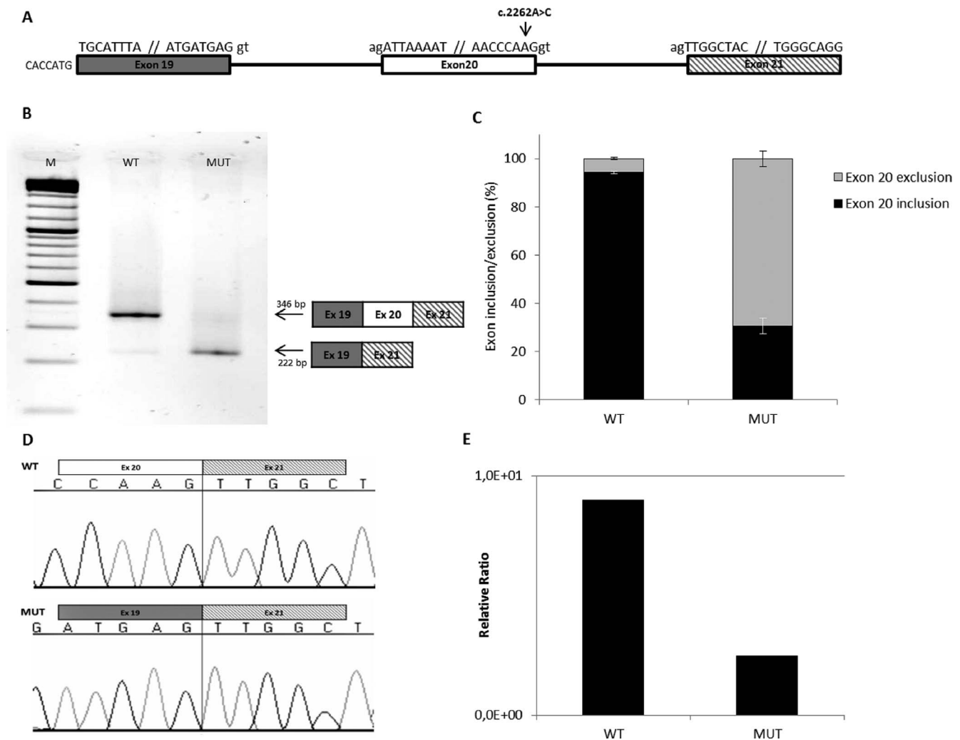
FIGURE. Splicing assay of DOCK9 . (A) Representation of the construct designed for the c.2262A>C variant in DOCK9 , including Kozak consensus (CACCATG) and exon ( uppercase letters ) and intron ( lowercase letters ) junction sequences. (B) Gel analysis of splice variants identified by RT-PCR on RNA extracted from transfected HeLa cells. WT, wild-type construct; MUT, mutated construct; M, ladder; 346 bp, normal transcript; 222 bp, aberrant transcript. (C) Histogram depicting the relative percentage (%) of each transcript calculated against the total intensity of the bands representing each isoform, using ImageJ. (D) Sequencing result of different bands obtained by PCR representing a normal product from the c.2262A allele and an aberrant product from the c.2262C allele with the exclusion of exon 20 of DOCK9 . (E) Quantitative real-time PCR analysis of DOCK9 mRNA in wild-type c.2262A and mutant c.2262C HeLa cells. Expression level was normalized to \beta -actin.
