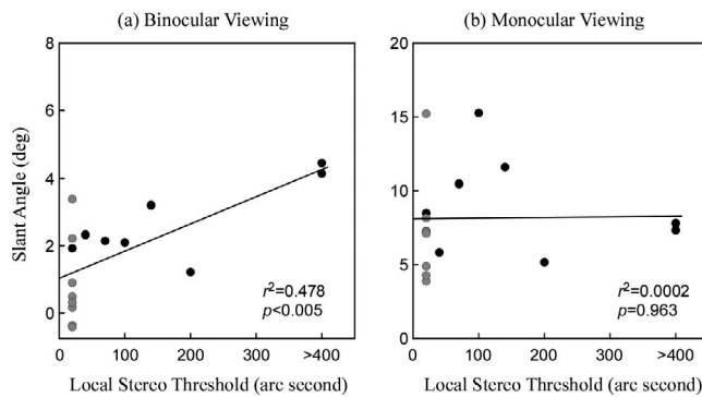
FIGURE 4. Slant angle as function of local stereo threshold (normal observers, gray circles ; strabismic observers, black circles ). The slant angle reliably increases with stereo threshold in the (a) binocular viewing condition, but not in the (b) monocular viewing condition.
