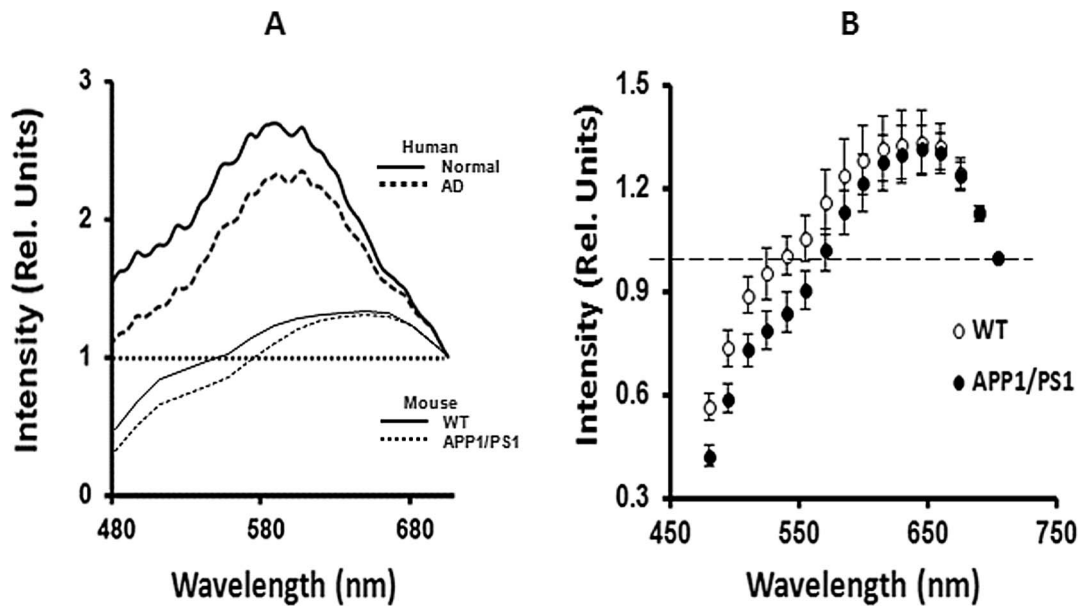
FIGURE 5. Optical spectra recorded from human and mouse retina samples. (A) Comparison of spectral shapes from Alzheimer's and normal retina (see the Results section). The upper curves show spectra from human retinal whole mounts, obtained postmortem from an individual diagnosed with AD ( n = 1 ) compared with a normal subject ( n = 1 ). Lower curves compare spectra obtained at 7 months from live APP1/PS1 mice and live WT mice ( n = 8 ). (B) Mice spectra from (A) shown with standard deviations at each wavelength. At wavelengths lower than 570 nm, error bars from each mean spectrum do not overlap.
