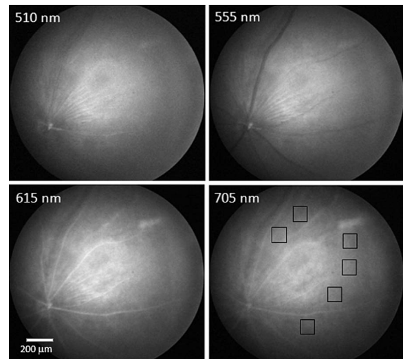
FIGURE 4. Monochromatic images from WT B6c3F1J mouse retina. Upper left: 510 nm (blue light) nerve fibers (center) and reflections from vessel below the fibers are bright. Upper right: 555 nm (green light), large vessels appear dark. Nerve fibers appear in center as bright. Veins are darker than arteries due to relatively greater absorbance of deoxyhemoglobin. Lower left: 615 nm (red light), arteries and veins both show brightly and nerve fibers are still visible. Lower right: 705 nm (near infrared), vessels and fibers lose brightness and deeper choroidal capillaries near center are in sharper focus. Boxes show locations typical of amyloid measurement areas.
