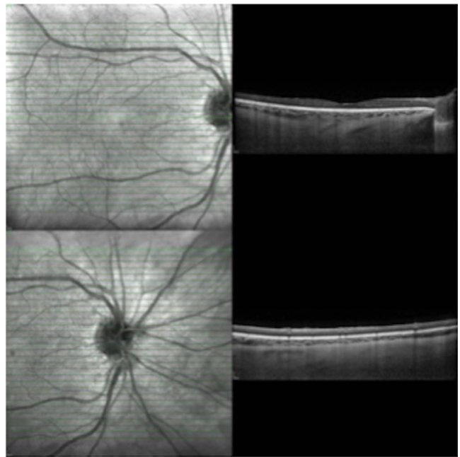
FIGURE 1. The OCT imaging protocol included volume scans of the macular region (centered on the fovea, top row ) and the peripapillary region (centered on the optic disc, bottom row ). As shown to the left of each OCT scan, the near-infrared image illustrates the size of the volume scans according to the predefined protocol. Corresponding fundus images were also obtained (not shown).
