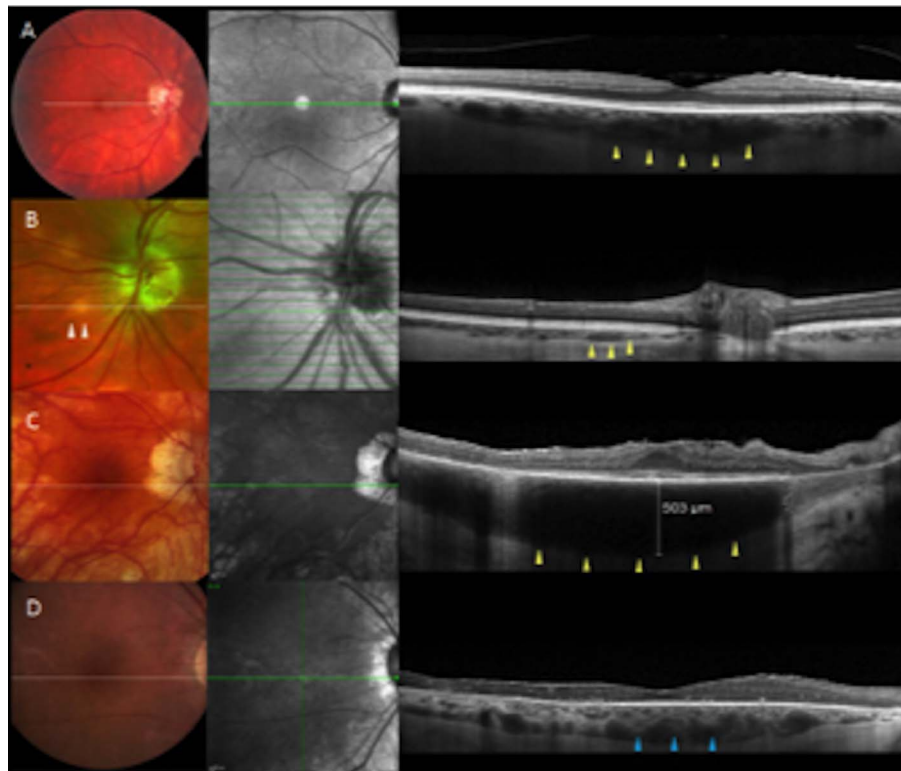
FIGURE 2. Four cases of birdshot chorioretinitis that illustrate relationships between OCT images (shown with the associated infrared image for each) and the corresponding fundus appearance, which may or may not reveal clinically apparent “birdshot lesions.” (Top row) OCT reveals a large hyporeflective choroidal lesion ( yellow arrowheads ) without a corresponding clinical lesion in the fundus photograph (A). (Second row) OCT shows a small, hyporeflective lesion in the inner choroid, just below the retinal pigment epithelium; the segmentation plane colocalizes at the position of a typical birdshot lesion on the fundus photograph (B, white arrowheads ). There is a notable absence of choroidal vascular markings. (Third row) OCT shows a large diffuse area of hyporeflectivity in an area of marked choroidal thickening ( yellow arrowheads ), without a corresponding clinically apparent lesion on the fundus photograph (C). This area of hyporeflectivity appears to represent a choroidal mass, possibly an infiltrate, that is blocking signal penetration. Note the presence of juxtapapillary retinal pigment epithelial atrophy, which allows increased transmission in the sclera and hyperreflectivity, despite the presence of a probable choroidal lesion, identified by thickening and loss of the normal choroidal vascular markings. (Fourth row) OCT shows hyporeflective areas associated with physiologic choroidal vessels ( blue arrowheads ) but no choroidal lesions as seen in the other scans.
