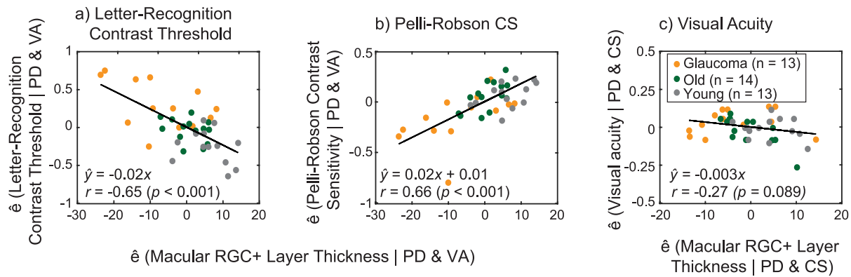
FIGURE 3. Partial correlations between functional and structural data after controlling for pupil diameter and visual acuity. In the partial correlation plot, \hat{e}(c|a,b) represents the residuals from the regression of the c variable on the a and b variable. The orange dots represent data from glaucoma patients ( n = 13 ), whereas the green and gray dots represent data for normal older adults ( n = 14 ) and young adults ( n = 13 ), respectively. The black lines represent the best linear fit to the data. (A) Correlation between letter-recognition contrast threshold and macular RGC+ layer thickness after regressing out the effects of pupil diameter (PD) and visual acuity (VA). (B) Correlation between Pelli-Robson contrast sensitivity (CS) and macular RGC+ layer thickness after regressing out the effects of PD and VA. (C) Correlation between visual acuity (logMAR) versus macular RGC+ layer thickness after regressing out the effects of PD and CS.
