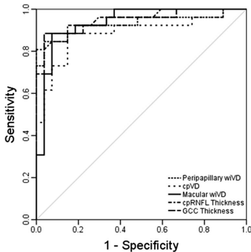
FIGURE 2. Area under the receiver operator characteristic curves of the peripapillary wiVD (0.93); cpVD (0.89); macular wiVD (0.94); cpRNFL thickness (0.95); and GCC thickness (0.95) for discriminating glaucomatous from healthy eyes.
