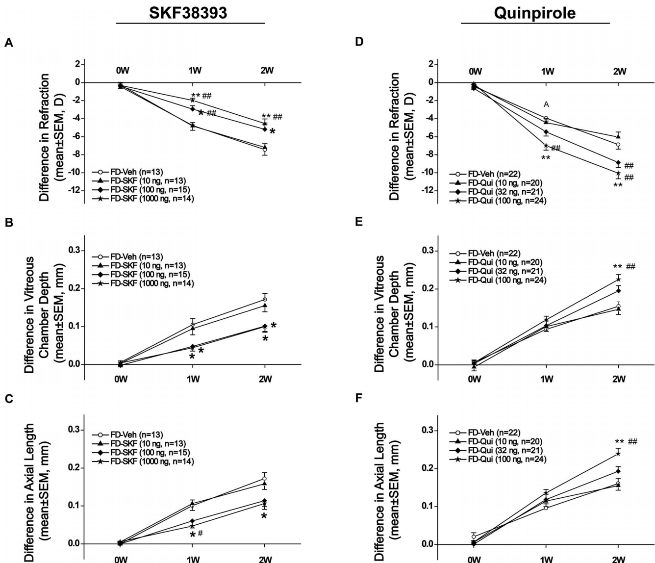
FIGURE 2. D1R and D2R agonists modulate refraction, VCD, and AL. SKF38393 inhibited, while quinpirole promoted, FDM progression. SKF38393 induced changes in the interocular differences in (A) refraction, (B) VCD, and (C) AL. FD-Veh, FD eyes treated with SKF38393 vehicle; FD-SKF, FD eyes treated with SKF38393. * P < 0.05 compared to FD-Veh; ** P < 0.01 compared to FD-Veh; # P < 0.05 , ## P < 0.01 , compared to the lowest-dose group (FD-SKF, 10 ng). Quinpirole induced changes in the interocular differences in (D) refraction, (E) VCD, and (F) AL. FD-Veh, FD eyes treated with quinpirole vehicle. FD-Qui, FD animals treated with quinpirole. * P < 0.05 compared to FD-Veh; ** P < 0.01 compared to FD-Veh; # P < 0.05 , ## P < 0.01 , compared to lowest-dose group (FD-Qui, 10 ng).
