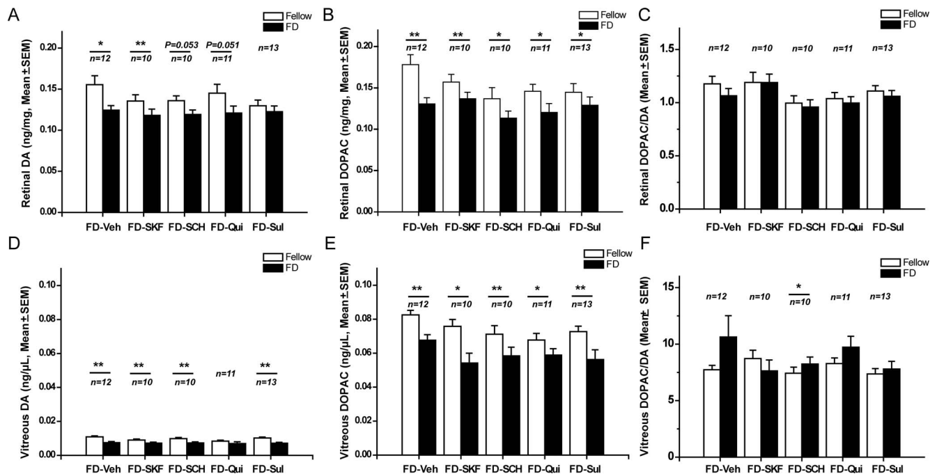
FIGURE 1. Effects of DR drugs on DA and DOPAC levels. FD decreased concentrations of DA and DOPAC in the retina and vitreous, but DR drugs did not alter DA turnover, as indicated by DOPAC/DA ratios in the retina and vitreous. (A) Retinal DA. (B) Retinal DOPAC. (C) Retinal DOPAC/DA ratio. (D) Vitreous DA. (E) Vitreous DOPAC. (F) Vitreous DOPAC/DA ratio. Open bar , fellow eye; solid bar , FD eye. SKF38393 (1 μg, FD-SKF, n = 10 ), SCH23390 (2500 ng, FD-SCH, n = 10 ), quinpirole (100 ng, FD-Qui, n = 11 ), and sulpiride (25 μg, FD-Sul, n = 13 ) injected (0.1 mL) into the inferior peribulbar space around FD eyes. One-way ANOVAs with Dunnett's post hoc test evaluated drug effects on DA, DOPAC concentration, and DOPAC/DA ratio, comparing drug- and vehicle-treated groups (all P > 0.05 ). Paired t -tests determined whether any of the differences in DA or DOPAC levels between treated and fellow eyes were significant (* P < 0.05 ; ** P < 0.01 ).
