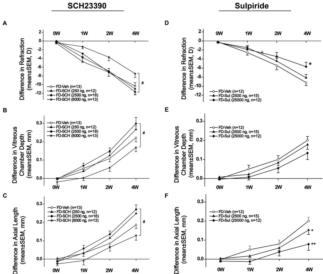
FIGURE 3. D1R and D2R antagonists modulate refraction, VCD, and AL. SCH23390 treatment had no effects on the interocular differences in refraction (A), VCD (B), and AL (C) of FD eyes compared with vehicle-treated eyes, at each time point. FD-Veh, SCH23390 VC undergoing FD. FD-SCH, FD animals treated with SCH23390. # P < 0.05 FD-SCH (2500 ng) compared to SCH (8000 ng). Sulpiride treatment inhibited FDM progression, as revealed by the declines in interocular differences in refraction (D), VCD (E), and AL (F) during FDM progression. FD-Veh, sulpiride VC undergoing FD. FD-Sul, FD animals treated with sulpiride. * P < 0.05 compared to FD-Veh. ** P < 0.01 compared to FD-Veh.
