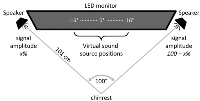
FIGURE 2. Apparatus for Experiment 2, stereo speakers with LED monitor. Phantom sources were generated at locations on the azimuth (auditory angle \theta ) between the two physical speakers by amplitude panning. The speakers were driven by coherent signals of independently variable amplitude, such that the signal amplitude gain to the right and left speakers always summed to 1.
