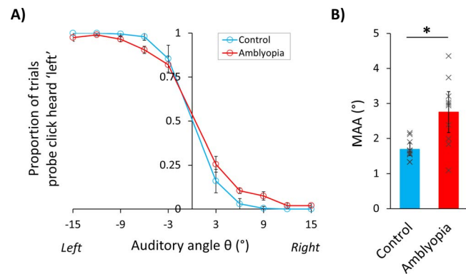
FIGURE 3. Relative sound localization performance on a horizontal speaker array. Error bars indicate \pm 1 SEM. (A) Mean psychometric data for the minimum audible angle task. Negative and positive auditory angles represent sounds presented to the left and right of the central click, respectively. (B) The mean minimum audible angle (MAA). The symbols (X) represent individual MAA values. The mean MAA was significantly larger in the amblyopia group compared with the control group ( *P = 0.006 ).
